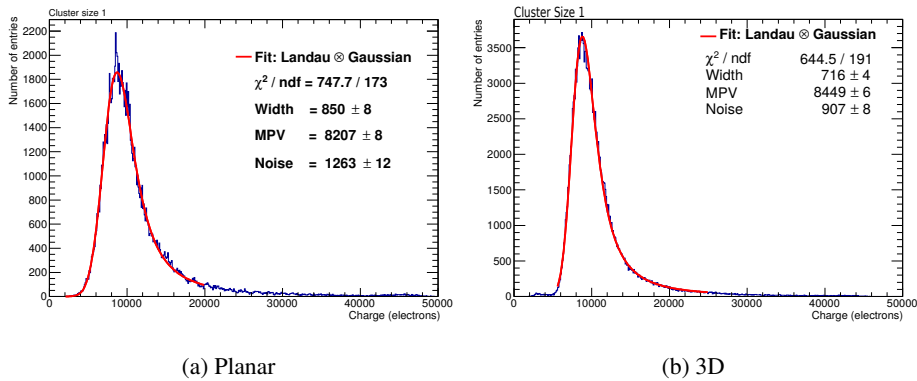
Figure 3: Collected charge distributions for a planar sensor operated at 100V (a) and a 3D sensor (b) operated at 40 V, with same active thickness ( 130\ \mu\text{m} ) [9].
