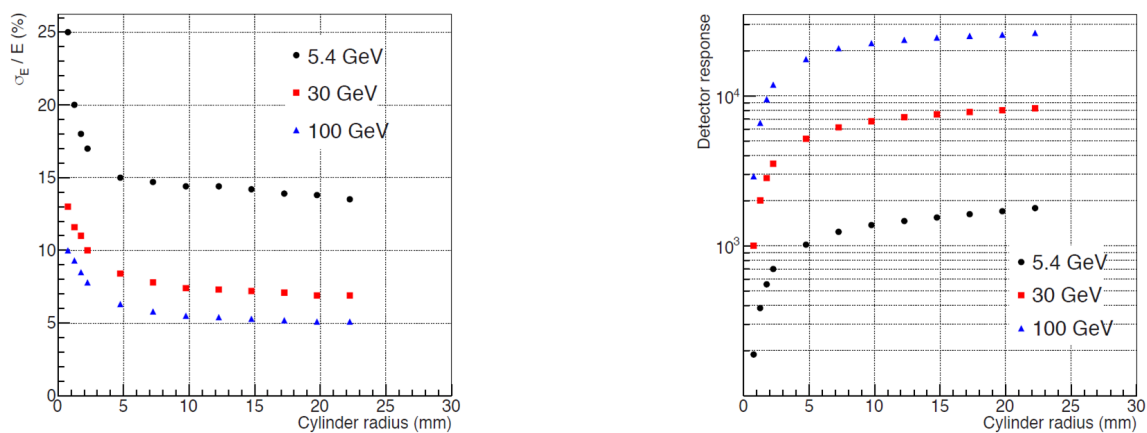
Figure 21. Resolution and response as a function of the radius of the core for different energies.
