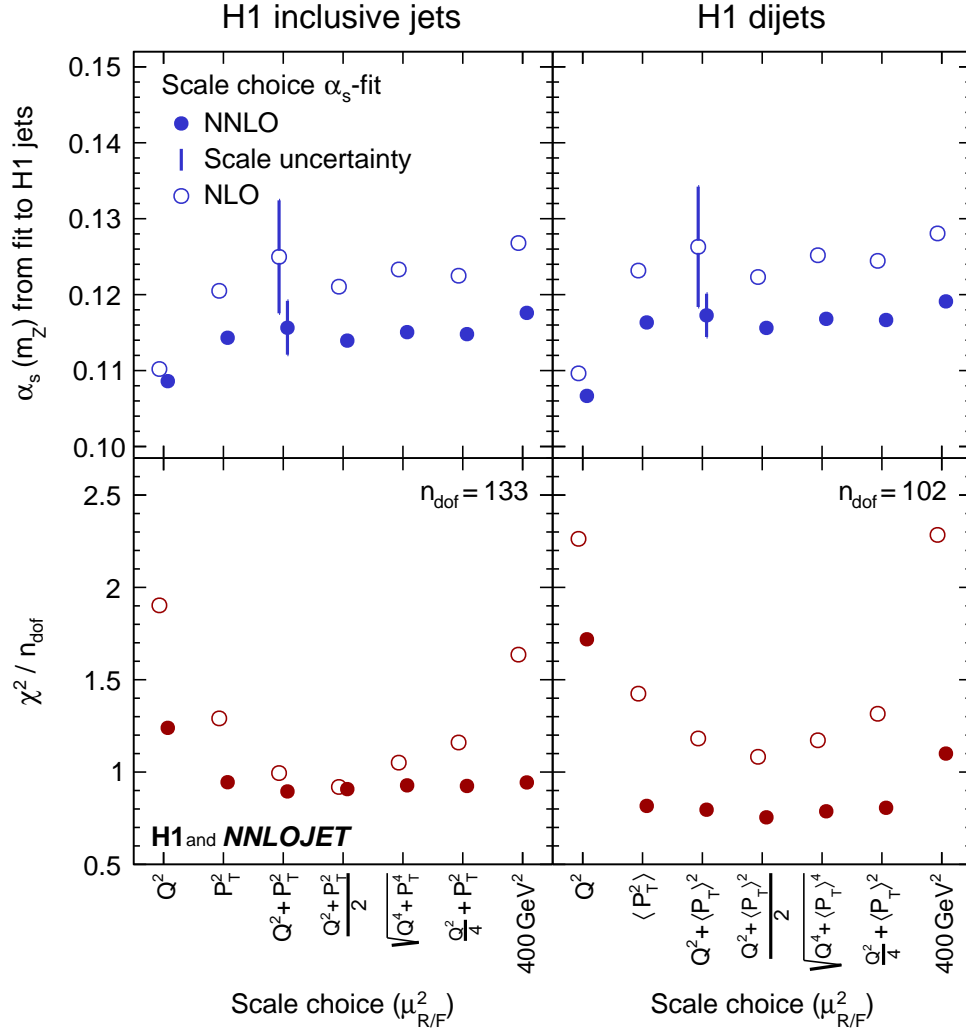
Figure 8: Values of \alpha_s(m_Z) obtained for different definitions of the renormalisation and factorisation scales ( \mu_R and \mu_F ) in separate fits of inclusive jet and dijet data. The lower panels show \chi^2/n_{\text{dof}} of the fits. The open circles display results obtained using NLO matrix elements. The vertical bars indicate the scale uncertainties displayed together with the nominal scale choice.
