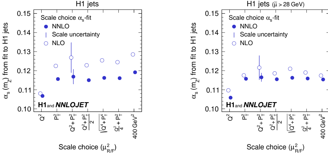
Figure 9: Values of \alpha_s(m_Z) obtained for different definitions of the renormalisation and factorisation scales ( \mu_R and \mu_F ) in the H1 jets fit (left) and the H1 jets fit with \tilde{\mu} > 28 GeV (right). The open circles display results obtained using NLO matrix elements. The vertical bars indicate the scale uncertainties displayed together with the nominal scale choice.
