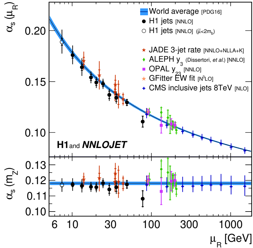
Figure 14: Results for \alpha_s(m_Z) and \alpha_s(\mu_R) for fits to data points arranged in groups of similar \mu_R , compared to results from other experiments and processes. Further details can be found in the caption of figure 13.
