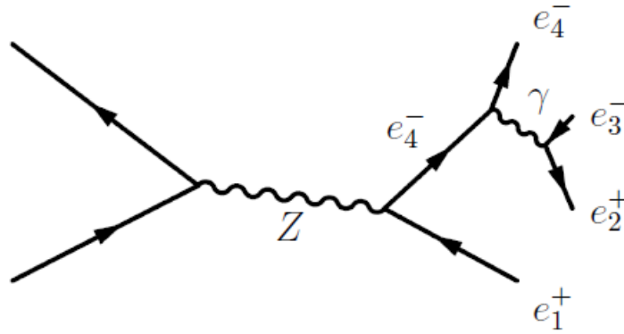
Figure 4.3.: Feynman graph showing the production of a Z -boson and the decay into two oppositely charged leptons (here electrons). One of the electrons radiates a photon, which converts into another lepton-antilepton pair.
