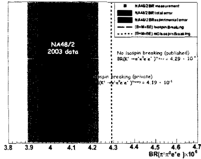
Figure 2 – The K^\pm \rightarrow \pi^\pm \pi^0 e^+ e^- branching ratio obtained by the NA48/2 2003 data sample is plotted with its experimental error (shaded blue band) and its total error (shaded green band). The total error included statistical, systematic and external errors. The small dashed line represents the theoretical prediction of the BR(K_{\pi\pi ee}) with no isospin breaking published in Ref. 2 . The big dashed line shows the expected branching ratio with isospin breaking (thanks to the authors of Ref. 2 , private communication). The experimental value of the BR(K_{\pi\pi ee}) is in a very good agreement with the theoretical predictions (within one standard deviation).
