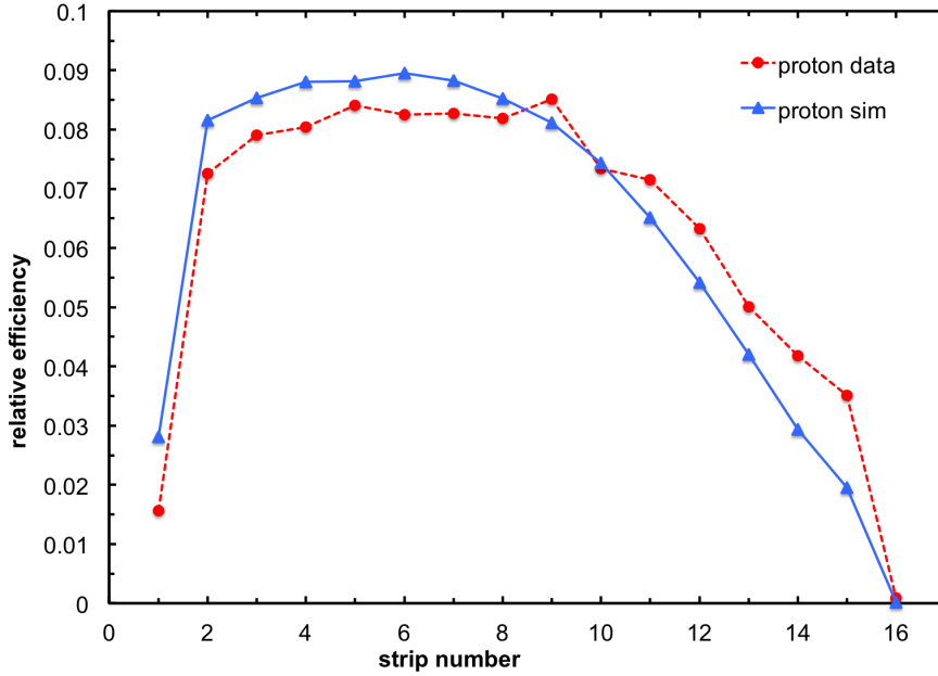
Figure 7. Relative detection efficiency of the setup, as a function of strip number, obtained in the GEANT4 simulation (isotropic emission was assumed) and with {}^7\text{Be} target (proton detection).
