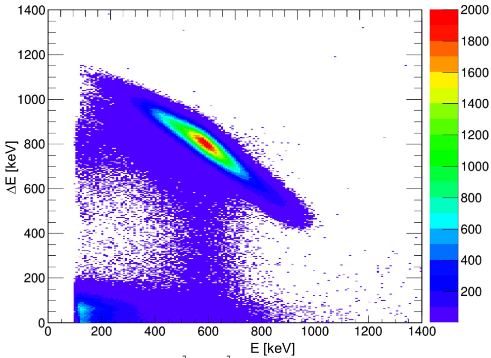
Figure 13. \Delta E - E scatter plot measured from the {}^7\text{Be}(n,p){}^7\text{Li} reaction, with the proton locus clearly visible.
