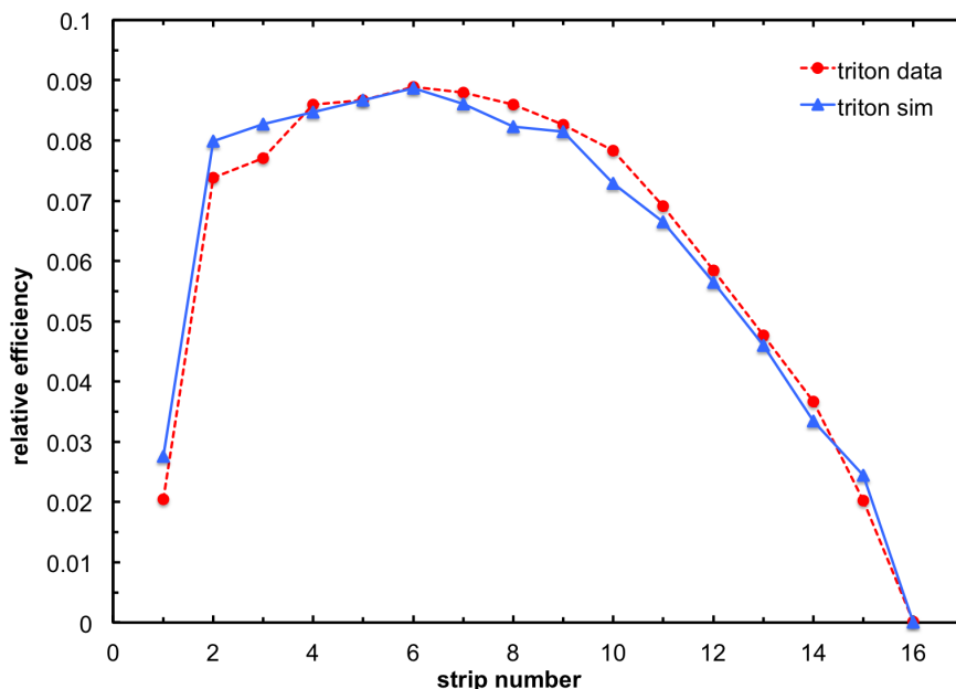
Figure 6. Relative detection efficiency of the setup, as a function of strip number, obtained in the GEANT4 simulation (isotropic emission was assumed) and with ^6\text{LiF} target (triton detection in the validation test).
