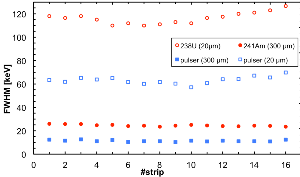
Figure 4. FWHM resolution for each \Delta E and E detector strip, tested with a pulser and with \alpha particles from ^{238}\text{U} (for the \Delta E detector) and ^{241}\text{Am} (for the E detector).
