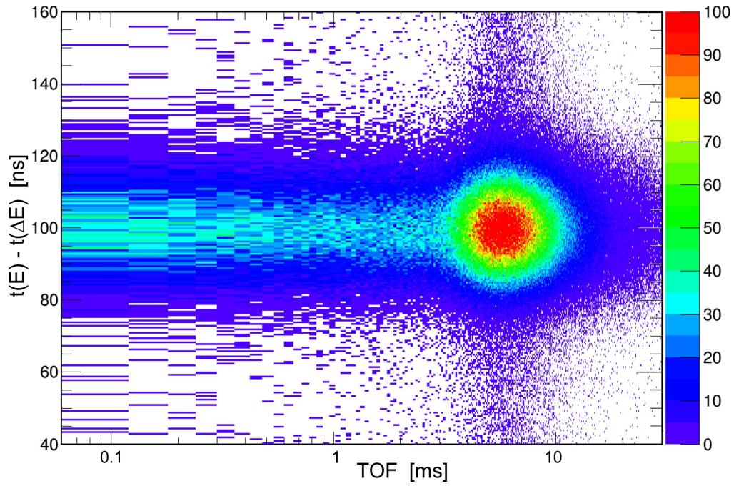
Figure 10. Scatter plot of the time interval between corresponding \Delta E and E strips in coincidence events as a function of the neutron time-of-flight, as measured in the {}^7\text{Be}(n,p){}^7\text{Li} reaction.
