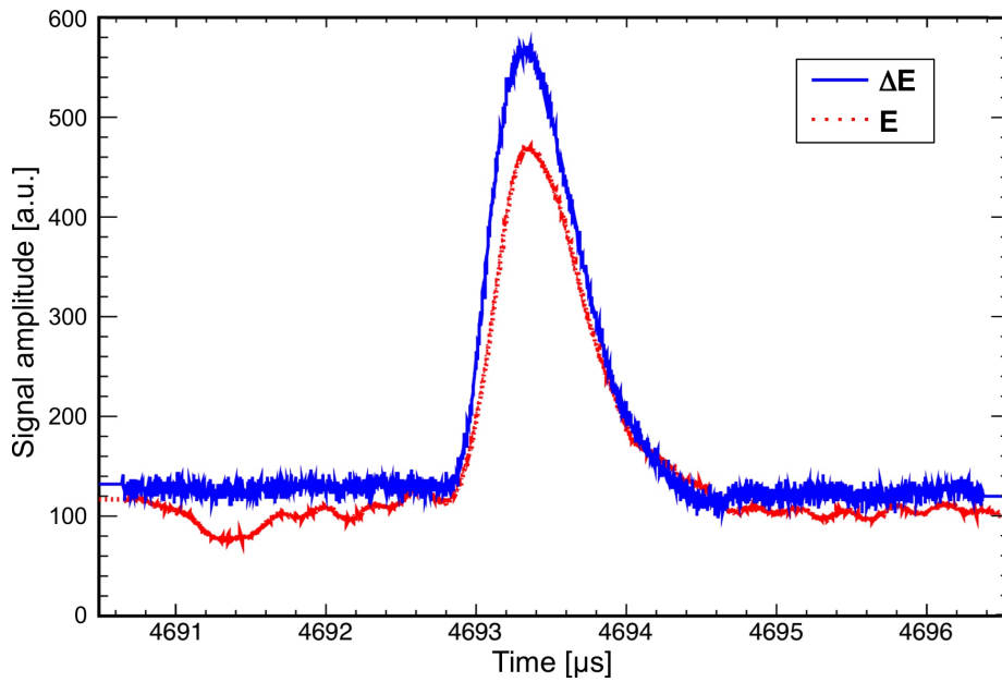
Figure 12. Snapshot of the \Delta E and E signals produced by a proton in a strip-strip coincidence event.
