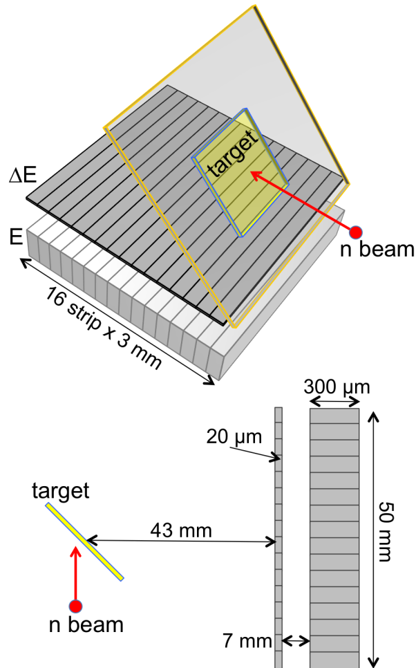
Figure 1. 3D sketch (top) and vertical profile (bottom) of the detector setup. The drawings are not to scale, and the \Delta E and E thicknesses are exaggerated for clarity.
