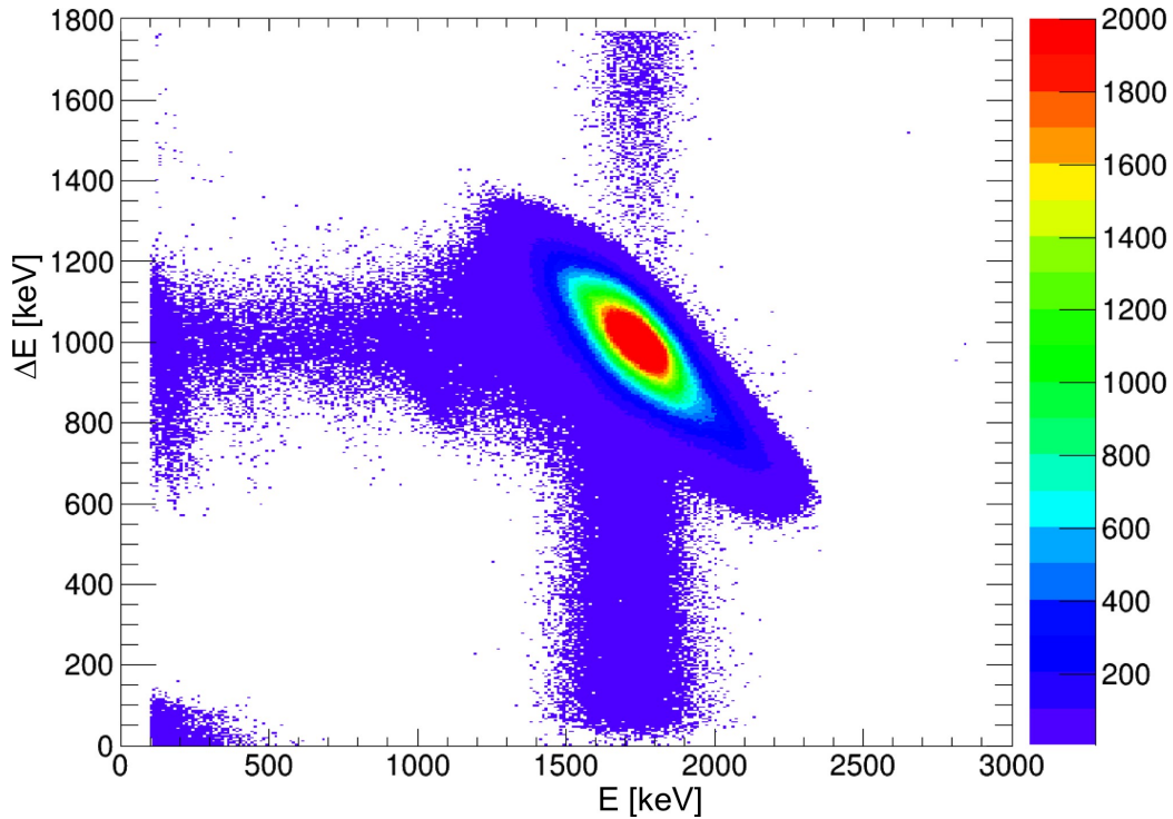
Figure 8. \Delta E - E scatter plot measured from the {}^6\text{Li}(n,\alpha) reaction, with the tritons locus clearly visible. The wide energy spread was due to the emission depth and angle in the target, and to the wide range of incidence angles on the detector.
