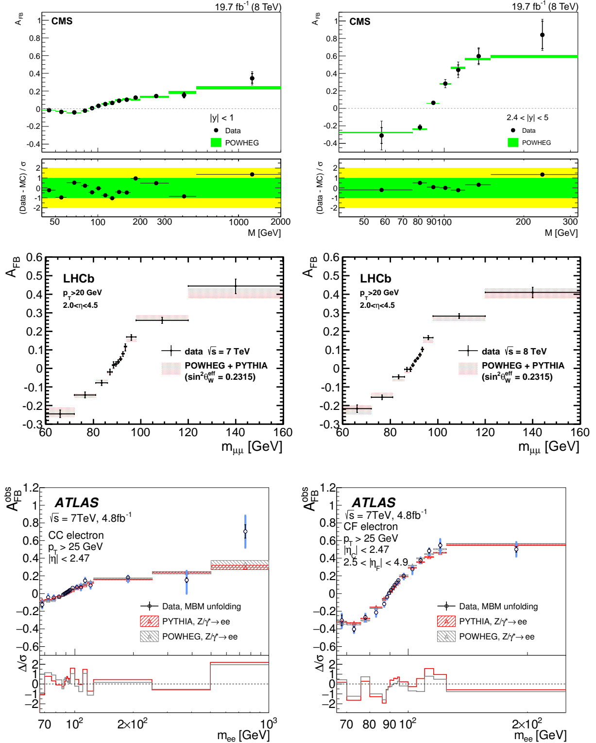
Figure 1 – Measured A_{FB} values in selected rapidity regions with the CMS 6 (top panel), LHCb 8 (middle panel), and ATLAS 11 (bottom panel) detectors. Inner (outer) vertical bars show the statistical (statistical plus systematic) uncertainties. The measurements are compared with POWHEG 12,13 and PYTHIA 14 predictions using the world average value of \sin^2 \theta_{\text{eff}}^{\text{lept}} . The shaded bands represent the uncertainties in the prediction described in the original articles 6,8,11 .
