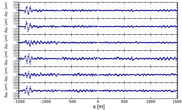
Figure 3: Leakage orbits in the vertical direction due to X-Y coupling in LER. After corrections. Kick angle of each horizontal steering is 200 \mu\text{rad} . Lambertson septum is located at s=-1400 m and s = 0 m indicates a location of IP.
