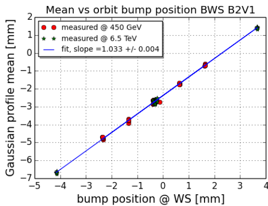
Figure 1: Gaussian profile mean of beam 2 vertical measured with wire scanner at different orbit bumps at 450 GeV (red) and 6.5 TeV (green), Fill 3644 (April 24, 2015). A linear fit (blue) is applied.
