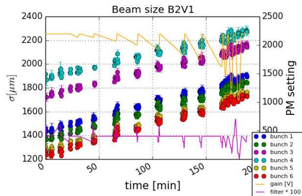
Figure 2: Beam 2 vertical beam size of six single bunches from wire scans at 450 GeV, Fill 3808 (May 31, 2015). The PM voltage (orange) and filter (purple) are displayed.
