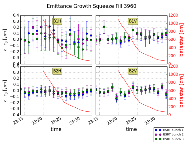
Figure 7: Emittance from BSRT measurements of three single bunches during the tune change at 6.5 TeV and the \beta^* squeeze to 80 cm in ATLAS/CMS, Fill 3960 (July 4, 2015). The \beta^* value (red) is displayed.
