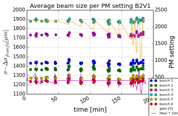
Figure 4: Average beam 2 vertical beam size per PM setting minus growth from exponential fit of six single bunches from wire scans at 450 GeV, Fill 3808 (May 31, 2015). The PM voltage (orange) and filter (purple) are displayed.
