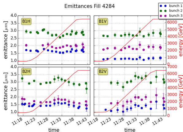
Figure 6: Emittance from wire scans of three bunches during the energy ramp to 6.5 TeV for Fill 4284. The energy (red) is displayed.
