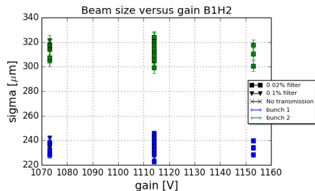
Figure 3: Beam 1 horizontal beam size of two single bunches from wire scans at 6.5 TeV, Fill 3809 (June 1, 2015), as a function of the applied PM voltage. The different PM filters are marked.
