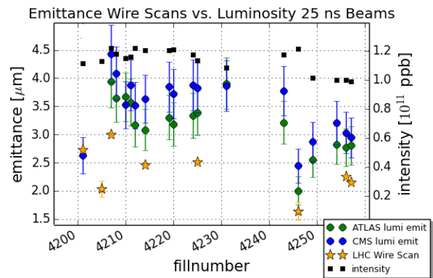
Figure 10: Emittance of 25 ns beams from ATLAS (green) and CMS (blue) luminosity at the start of collisions compared to the convoluted emittance at LHC injection measured with wire scanners (orange).
