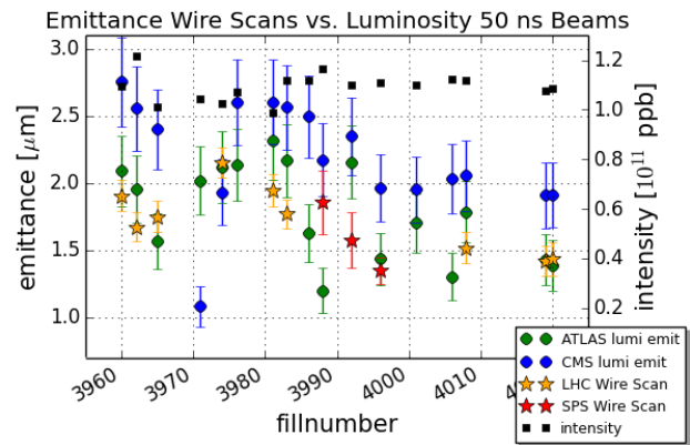
Figure 9: Emittance of 50 ns beams from ATLAS (green) and CMS (blue) luminosity at the start of collisions compared to the convoluted emittance at LHC injection (orange) or SPS extraction (red) measured with wire scanners.
