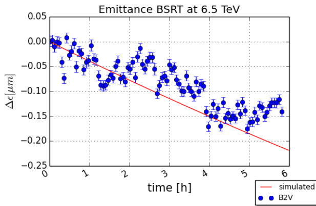
Figure 8: BSRT measurements of beam 2 vertical emittance during collisions of Fill 3988 (July 12, 2015) compared to simulations.
