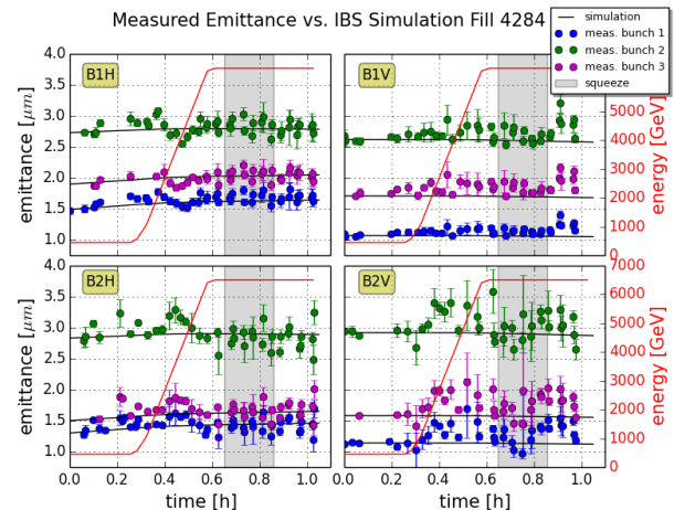
Figure 5: Emittance from wire scans of three single bunches during the LHC cycle, Fill 4284 (August 28, 2015), with IBS simulations (black). The energy (red) and \beta^* squeeze (grey) are displayed.
