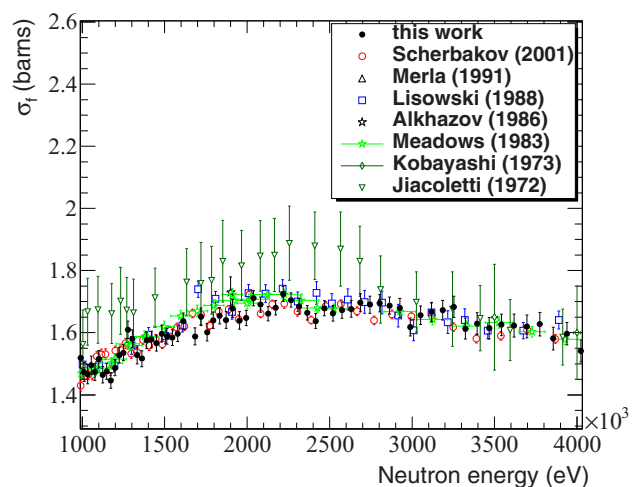
FIG. 9. Comparison of the present data with selected data from the EXFOR database [1], in the neutron energy range 1–4 MeV.
