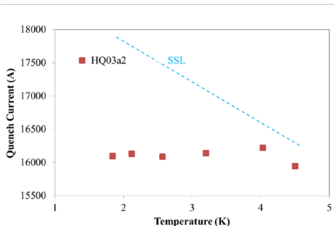
Fig. 3: Dependence of the quench current on temperature.
