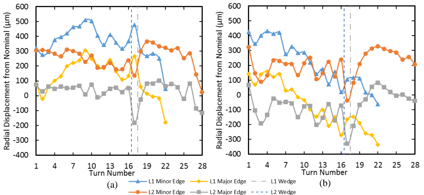
Fig. 7. Radial Turn Displacements with respect to the designed turn location. Figure 7(a) and 7(b) are the radial displacements for LARP coil 1 and CERN coil 101. L1 and L2 represent the inner and outer coil layers. Radially outward is considered a positive shift. Turn 1 is the midplane turn. The average displacement between the transition and non-transitions sides of a full coil cross section is presented. The minor and major edges of each layer track well. The difference between the minor and major edge is due to the less than expected width growth with respect to nominal.
