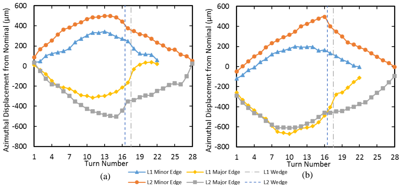
Fig. 6. Azimuthal Turn Displacements with respect to the designed turn location. Figure 6(a) and 6(b) are the azimuthal displacements for LARP coil 1 and CERN coil 101. L1 and L2 represent the inner and outer coil layers and Minor/Major indicate the cable edge displaced. Azimuthally toward the coil midplane is considered a positive shift. Turn 1 is the midplane turn. The average displacements between the transition and non-transitions sides of full coil cross section are presented.
