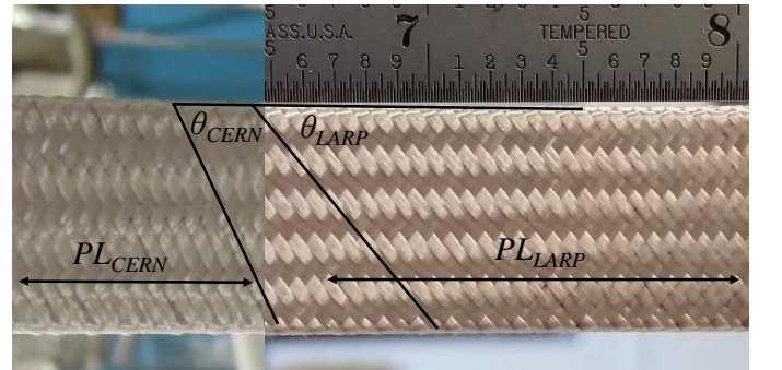
Fig. 4. Two types of braided-on insulation for MQXF. The pitch length and pitch angle are indicated. The insulation thicknesses are equivalent. The fiducial is in inches.
