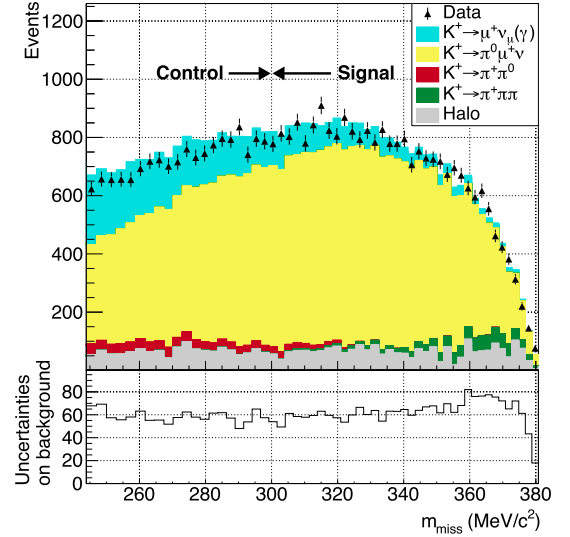
Fig. 3. Missing mass distributions for data, showing statistical uncertainties, and for the estimated background contributions, in both signal and control regions. The lower plot shows the total uncertainty on the background estimate.
