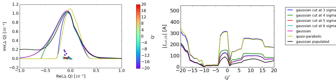
Figure 3. Effects of the tails of the transverse beam profiles on the single-beam stability just before putting beams in collision with the current HL-LHC impedance model: (left) stability diagram with the coherent modes inside and (right) required Landau octupoles current vs. chromaticity to reach beam stability.
