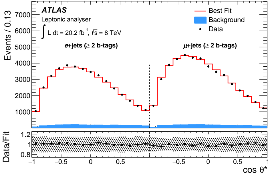
Figure 3: Post-fit distribution of \cos \theta^* for the leptonic analyser with \geq 2 b -tags, in which a two-channel combination is performed (electron and muon). The uncertainty band represents the total uncertainty in the fit result.
