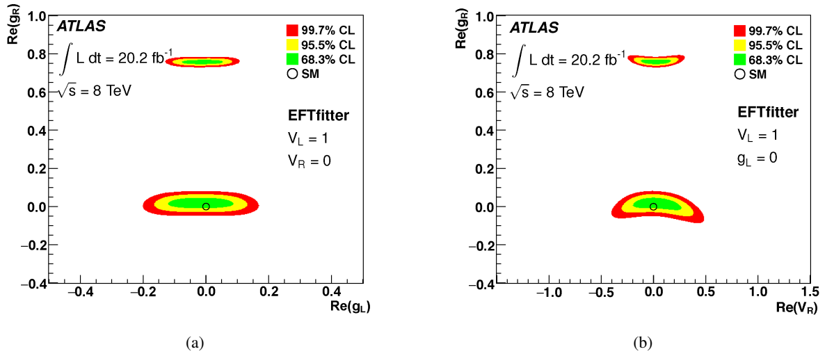
Figure 5: (a) Limits on the anomalous left- and right-handed tensor couplings of the Wtb decay vertex as obtained from the measured W boson helicity fractions from the leptonic analyser. (b) Limits on the right-handed vector and tensor coupling. As the couplings are assumed to be real, the real part corresponds to the magnitude. Unconsidered couplings are fixed to their SM values.
