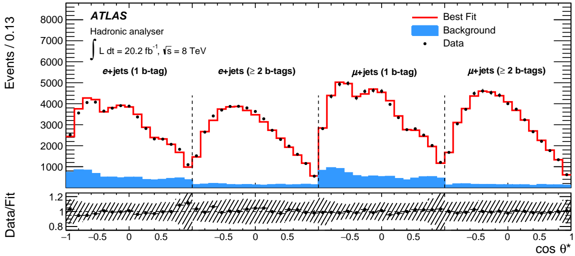
Figure 4: Post-fit distribution of \cos \theta^* for the hadronic analyser, in which the combination of four channels is performed (electron and muon, with exactly 1 b -tag and \geq 2 b -tags). The uncertainty band represents the total uncertainty in the fit result.
