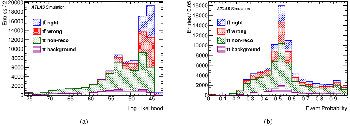
Figure 1: (a) Logarithm of the likelihood value as output for reconstructed t\bar{t} events. (b) Event probability for the selected (best) jet-to-parton permutation. Events from a t\bar{t} signal sample are split into events where the t\bar{t} pairs do not decay via the lepton+jets channel (“ t\bar{t} background”), events where not all t\bar{t} decay products have been reconstructed (“ t\bar{t} non-reco”), as well as correctly (“ t\bar{t} right”) and incorrectly (“ t\bar{t} wrong”) reconstructed t\bar{t} systems.
