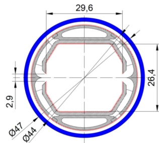
Figure 10: FCC-hh beam-screen design with integrated “folded” antechamber [16, 17].
