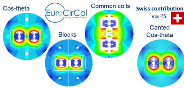
Figure 13: Four different design concepts for 16 T magnets.
