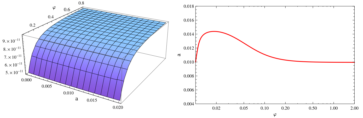
Fig. 1. The scalar potential V_E in the Einstein frame (left) and the inflaton trajectory (right). Here, we have fixed the parameters as \xi = 252 , \xi_A = -68 , m = \frac{y}{\sqrt{2}}M_G and m_A = \frac{y}{2\sqrt{2}}M_G with y = 0.01 and M_G = 0.01 (typical GUT scale).
