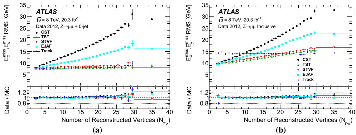
Fig. 7 The resolution obtained from the combined distribution of E_T^{\text{miss}} and E_V^{\text{miss}} for the CST, STVF, EJAF, TST, and Track E_T^{\text{miss}} algorithms as a function of N_{PV} in a 0-jet and b inclusive Z \rightarrow \mu\mu events
