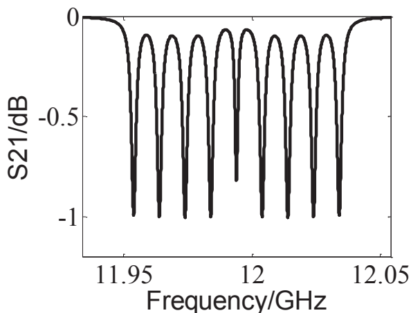
Figure 6: The spectrum of the second stage. The output pulse length is 100ns and the frequency difference between the two nearby peaks is 10MHz.
