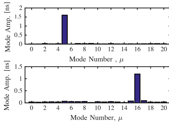
Figure 3: Mode amplitude for the uniform filling pattern, following the excitation of h_{CB} = 16 LSB (top) and USB (bottom).
