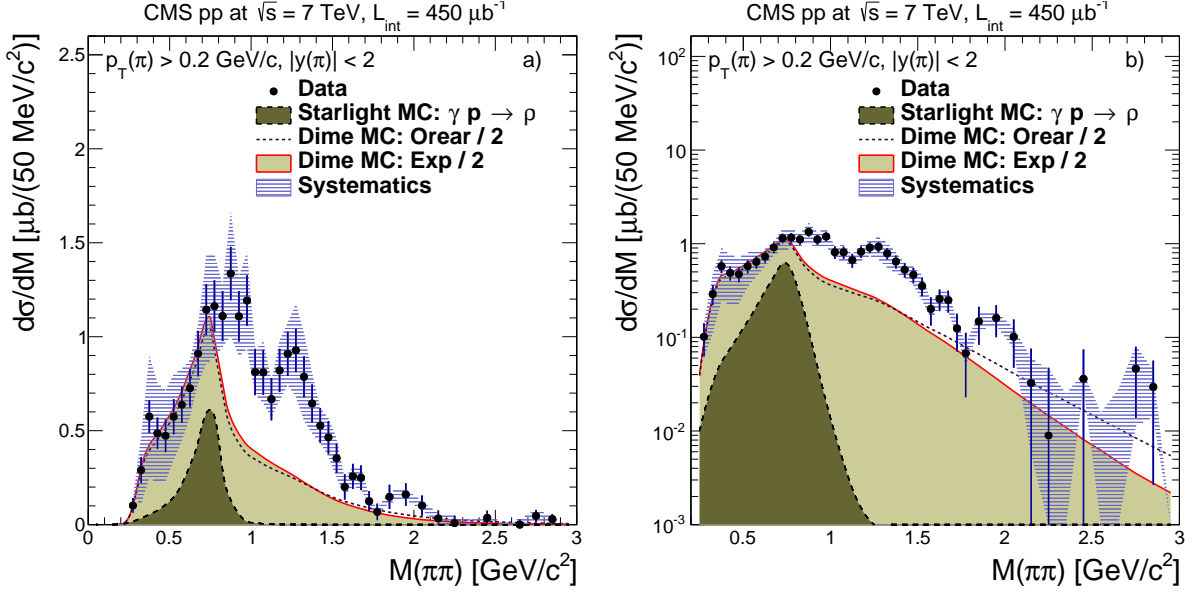
Figure 3: Corrected differential cross sections for pp \rightarrow p^{(*)}\pi^+\pi^-p^{(*)} as a function of dipion invariant-mass, compared to the stacked predictions of DPE production from the DIME MC (solid curve) and of \rho photoproduction from STARLIGHT (dashed curve). The shaded band shows the overall systematic uncertainty, and the error bar indicates the statistical uncertainty. The results are plotted on a linear scale (a) and a logarithmic scale (b).
