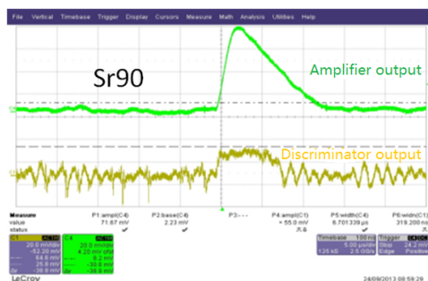
(a) Amplifier and comparator signals of Sr90.
