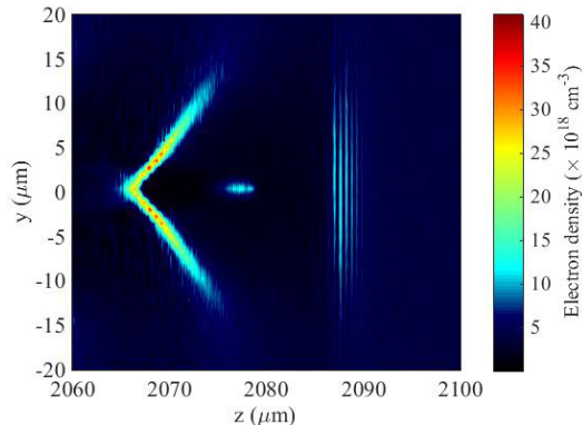
Figure 4: Electron density of the plasma at 7 ps after the laser pulse travelled in the plasma.
