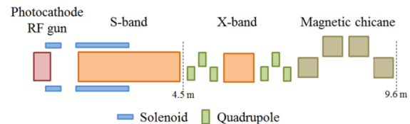
Figure 1: Layout of the RF-driven radiation source.
