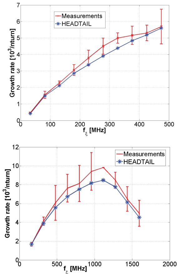
Figure 2: Comparison between measurements and simulations of the headtail vertical growth rates for both Q20 (top) and Q26 (bottom) optics.
