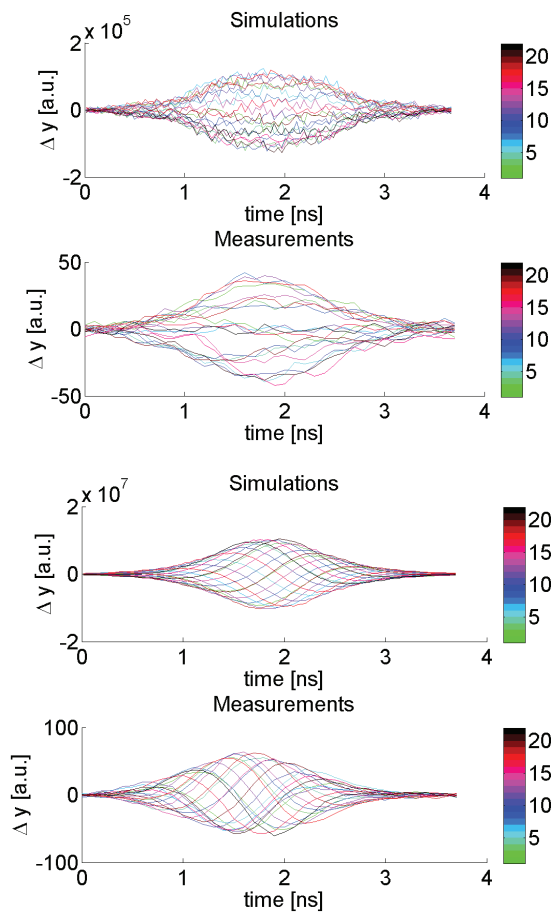
Figure 3: Comparison between measurements and simulations of the intra-bunch motion over 21 consecutive turns for \xi = -0.067 (top) and \xi = -0.967 (bottom).
