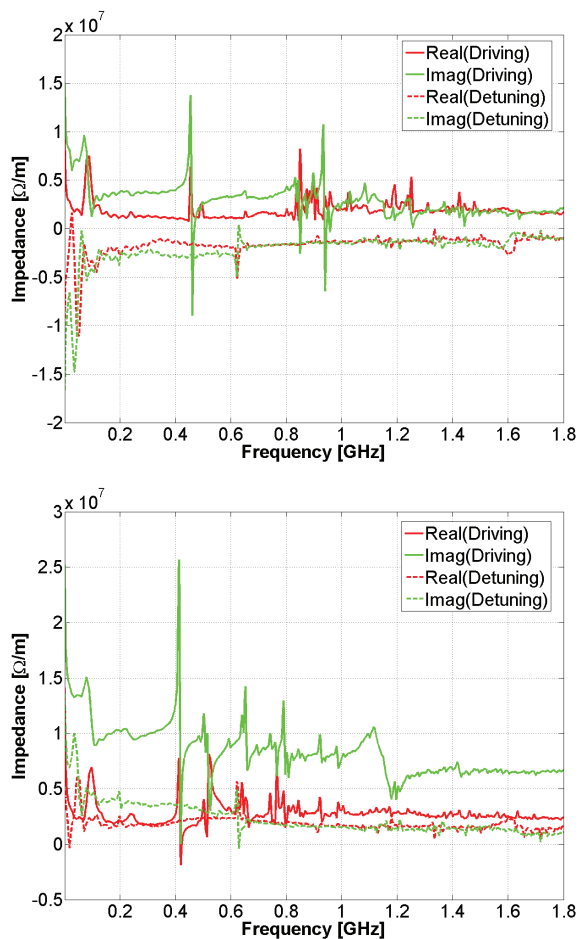
Figure 1: Horizontal (top) and vertical (bottom) SPS impedance model.
