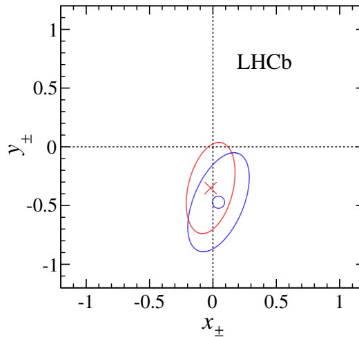
FIG. 9. Contours at 68% CL for the (blue) (x_+, y_+) and (red) (x_-, y_-) parameters associated with the B^0 \rightarrow DK^*(892)^0 decay, with statistical uncertainties only. The central values are marked by a circle and a cross, respectively.
