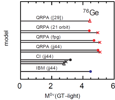
Fig. 8: The 0\nu NME for the light-neutrino decay of ^{76}\text{Ge} . See captions to Figs. 2 and 3.
