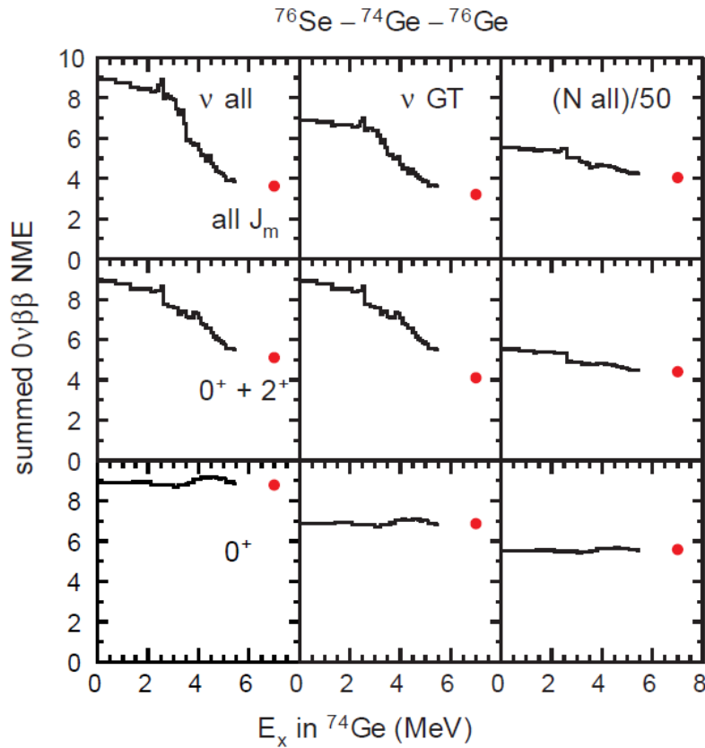
Fig. 3: Expansion of the NME over intermediate states ^{74}\text{Ge} .
