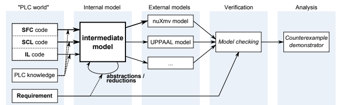
Figure 1. Overview of our approach
