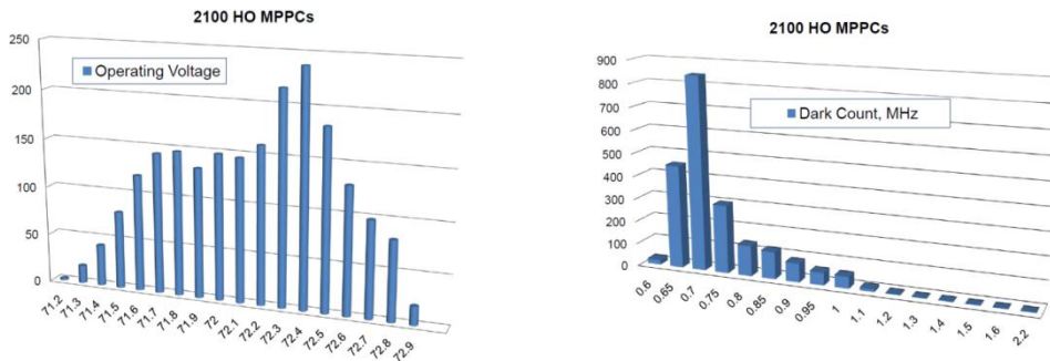
Fig. 5 (a) Variation in operating voltage for 2100 MPPCs; (b) Variation in dark count for 2100 MPPCs.
