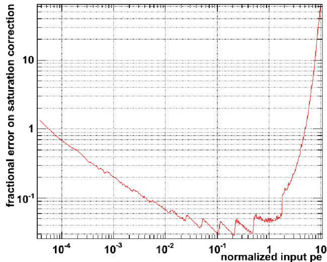
Figure 6. Fractional error (simulated) for the digitized QIE signal as a function of number of pes per MPPC micro-pixel.
