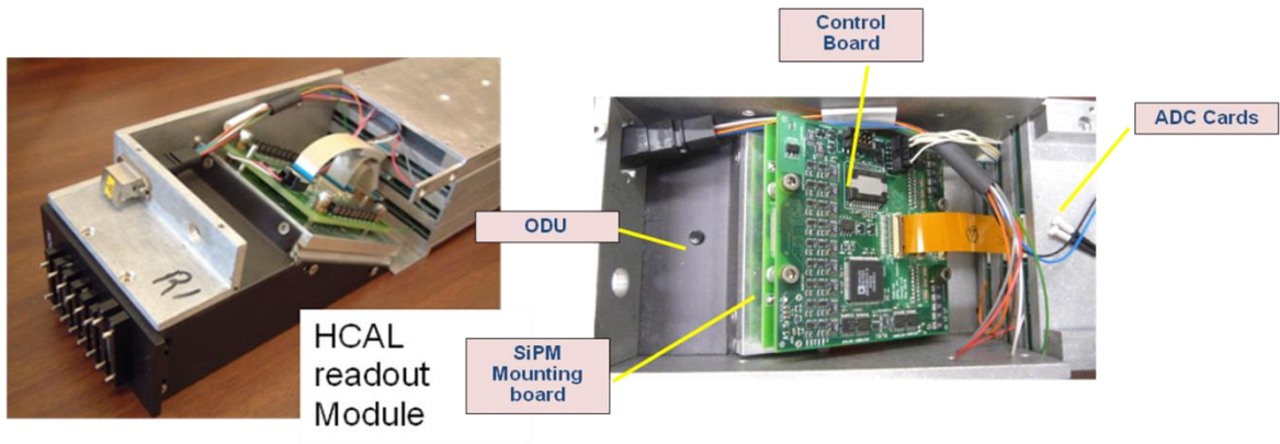
Figure 8a) and (b) Views of an opened RM where the Control Board (CB) is seen in (b). Also note the connection to the ADC cards (QIEs).
