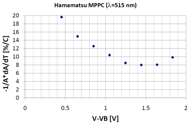
Figure 4. Variation in gain vs overvoltage for the MPPC.
