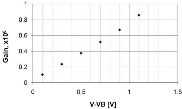
Fig. 3. Gain as a function of applied overvoltage for the MPPC;
