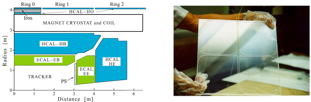
Fig. 1(a). Diagram of quarter section of CMS showing the location of the HCAL HO; 1(b) A HO scintillator tile.
