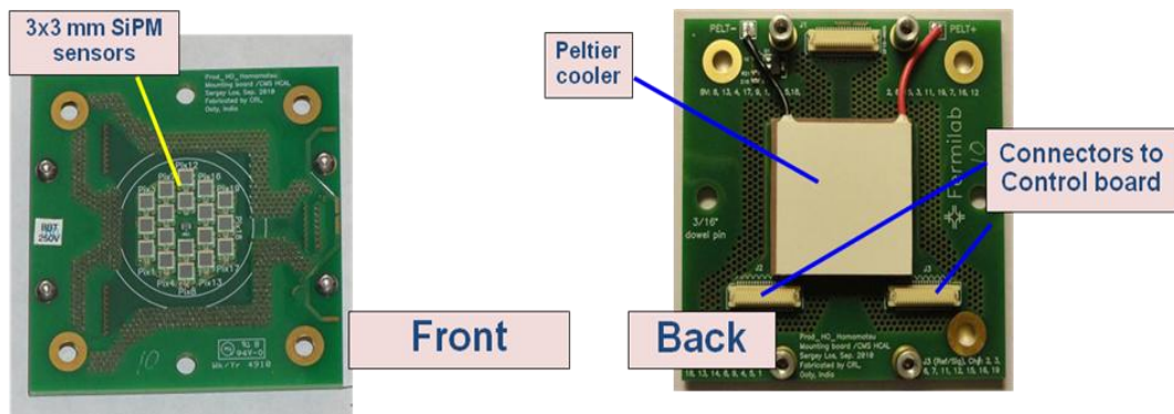
Figure 7. Photographs of the two sides of the Mounting Board (MB).
