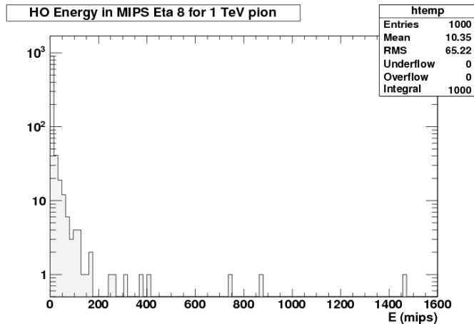
Figure 2. Energy deposition in MIPs into HO for 1000 GeV pions. One MIP corresponds to about 12 pes.
