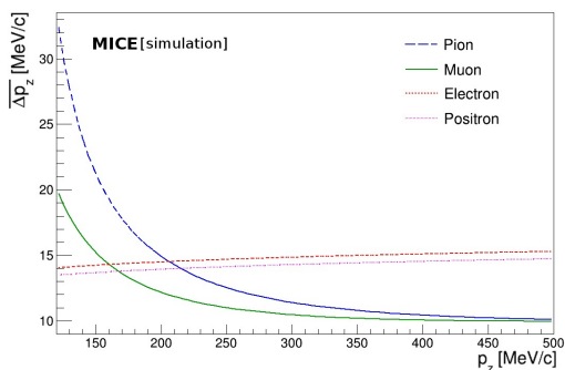
Figure 6. Continuous Slowing Down Approximation of the mean momentum loss ( \overline{\Delta p_z} ) of particles crossing TOF2 with impinging momentum p_z .
