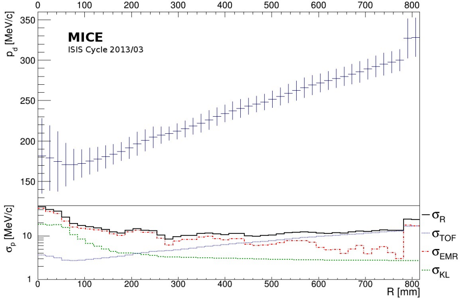
Figure 19. Downstream momentum ( p_d ) as a function of the range ( R ) in the EMR. A bin corresponds to a plane and its error bar represents the RMS of the momentum distribution within the bin.
