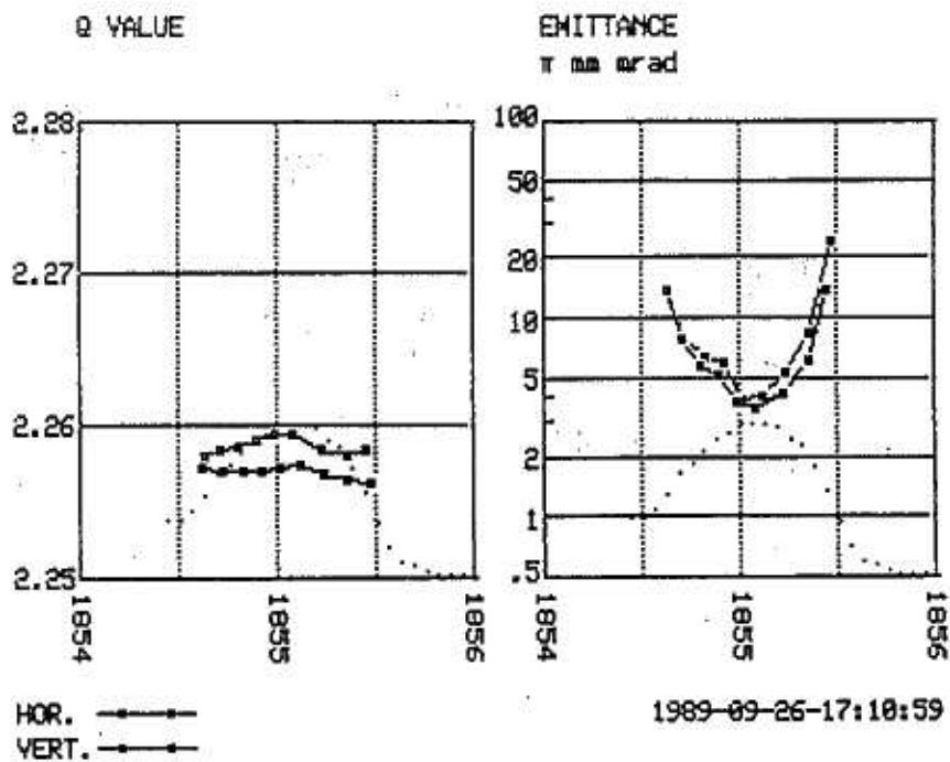
Fig. 4. Stack core Tunes and Emittances
