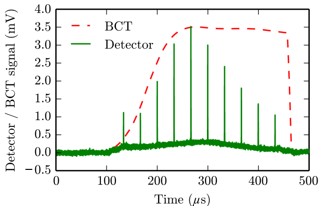
FIG. 11. Unamplified signal from a diamond detector channel sampling the H^0 particles for a given laser position ( E_{\text{pulse}} = 67 \mu\text{J} ; f_{\text{pulse}} = 30 \text{ kHz} ), as function of time along the 3 MeV H^- beam pulse. This is compared to the beam current measured with a beam current transformer (BCT) downstream the laser station.
