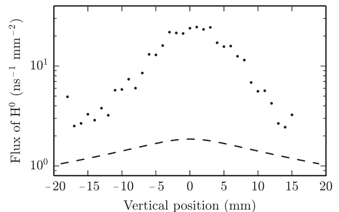
FIG. 3. Flux of H^0 arriving at the detection plane from laser stripping in the center of the H^- beam—in average while laser pulse duration—(dots); H^0 flux from the residual gas background—permanently while macro-pulse—(dashed line).
