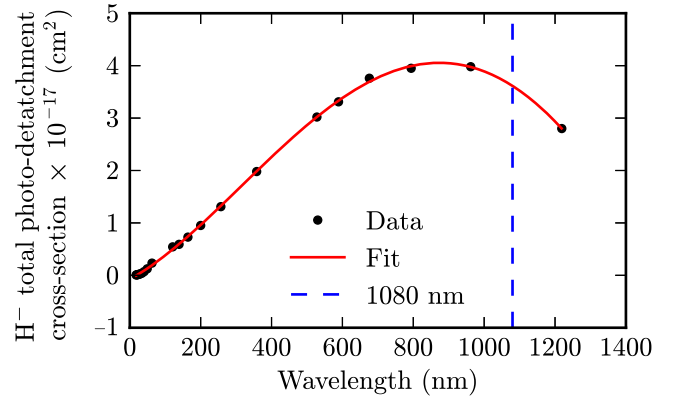
FIG. 2. Cross-section of the photo-detachment process of a nonrelativistic H^- ion. The dashed line indicates the selected laser wavelength for the emittance measurements at 3 MeV.
