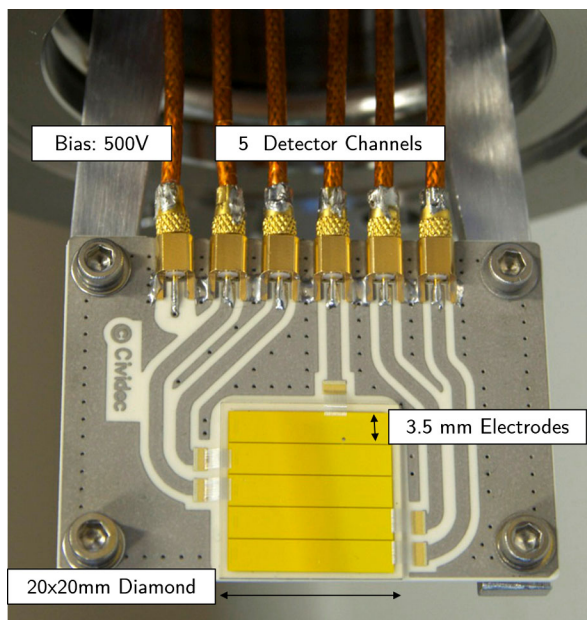
FIG. 7. pCVD diamond detector with 5 strip electrodes [21].
