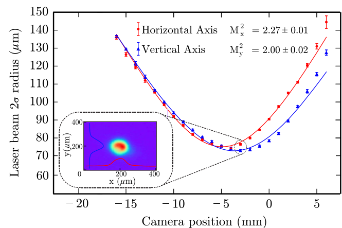
FIG. 8. Measured 2\sigma width of the laser beam focused by a lens with a focal length f = 500 mm. At the bottom left is shown the laser spot image taken at a position of -3 mm, where the minimum vertical size is obtained.
