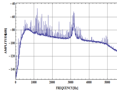
Figure 4: Horizontal spectrum during an LHC operation.
