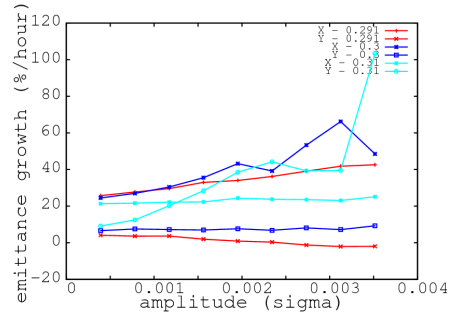
Figure 3: Emittance growth rate as a function of modulation amplitude at different modulation frequencies.
