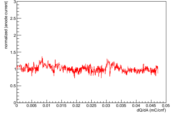
Figure 4: Variation of normalised |anode current| as a function dQ/dA.
