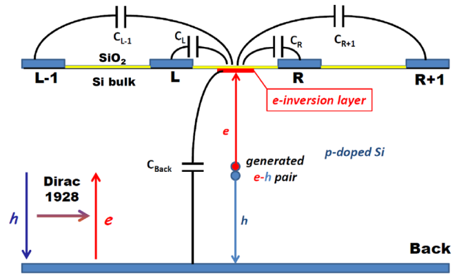
Fig. 13. Capacitance model of a strip sensor used to discuss charge sharing and charge losses in segmented silicon sensors. The insert Dirac 1928 is a reminder that an electron with momentum \vec{p} is equivalent to its antiparticle with momentum -\vec{p} .
