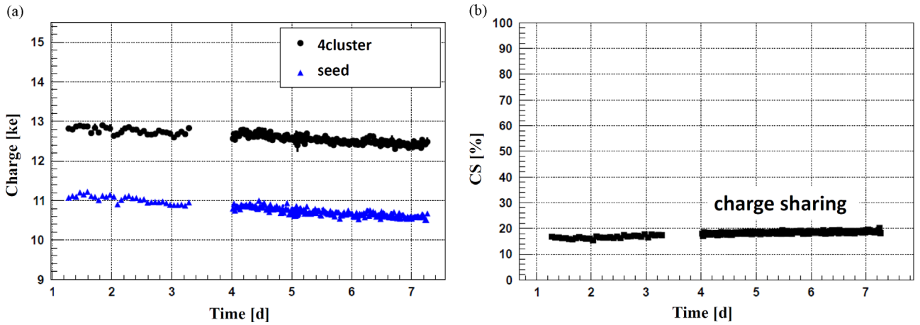
Fig. 10. (a) Median of the PH(4-cluster) and PH(seed) distributions for the FZ p -stop sensor irradiated by 15 \times 10^{14} n_{eq}/cm^2 24 GeV/c protons and 6 \times 10^{14} n_{eq}/cm^2 reactor neutrons as a function of the measurement time, during which the dose in the SiO 2 from the \beta source increased from 0 to 375 Gy(SiO 2 ). The applied voltage was 1000 V. (b) The corresponding time dependence for CS.
