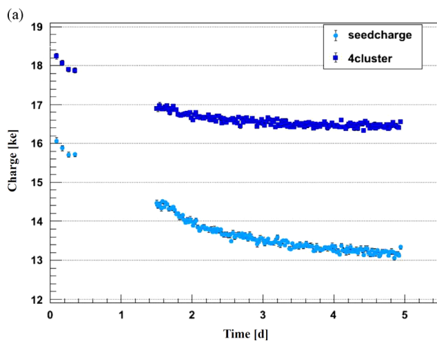
Fig. 8. (a) Median of the PH(4-cluster) and PH(seed) distributions for the non-hadron-irradiated p -spray sensor biased at 600 V as a function of the time from the beginning of the irradiation. The initial dose is 0 Gy and the dose after 5 days, 250 Gy( \text{SiO}_2 ). Between 0.4 and 1.4 days the measurement was interrupted because of a problem with the nitrogen flow, which is needed to prevent ice formation on the sensor at -20 °C. During that time the sensor remained exposed to the \beta source. (b) The corresponding time dependence for CS.
