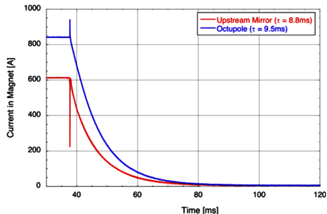
Fig. 25. Magnet quench shutdown comparison of the octupole ( \tau=9.5 ms) and the upstream mirror ( \tau=8.8 ms).
