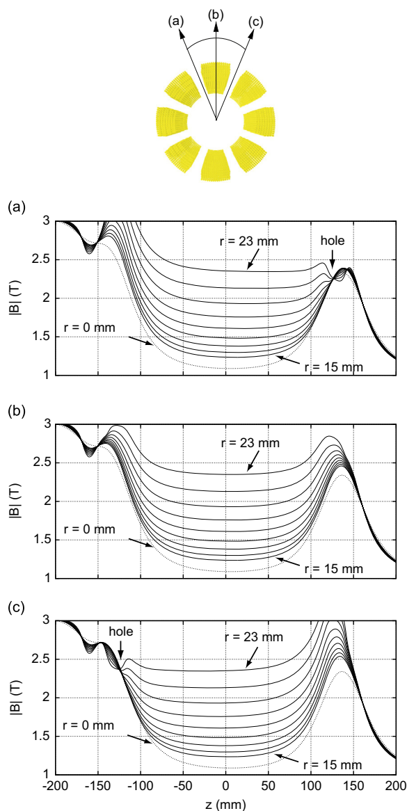
Fig. 11. The upper drawing is an axial view of a cross-section in the middle of the magnet system indicating the azimuthal angles for the planes for (a), (b) and (c). These three plots show the total field for a number of different radii as function of z . The radius for subsequent solid lines differs by 1 mm. (a) -22.5^\circ ; (b) 0^\circ ; (c) 22.5^\circ [20].
