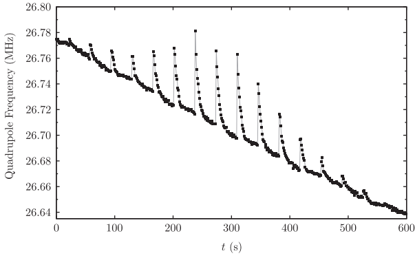
Fig. 29. Real-time readout of the quadrupole mode frequency of an electron plasma as a train of microwave pulses are applied, scanning across the cyclotron resonance in 1 MHz steps. The quadrupole mode frequency is measured roughly once per second. The overall linear decay of the quadrupole frequency is consistent with the slow expansion of the electron plasma.
