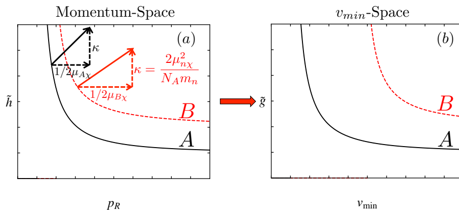
Figure 1. (a) A schematic of the momentum-space plot proposed in this work for two different detectors with target nuclei masses satisfying M_A > M_B . (b) A schematic of the standard v_{\min} -space plot. The mapping from the unique momentum-space plot to the v_{\min} -space plot is also shown in (a) for a typical choice of DM mass making clear that the differences only arise in the horizontal direction, see eq. (3.5).
