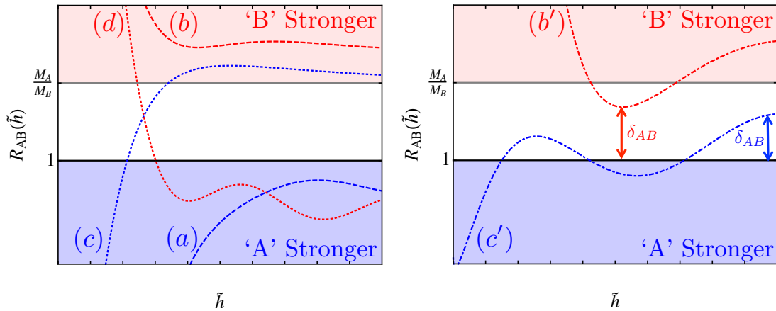
Figure 7. Some possibilities for the variable R_{AB} defined in eq. (A.1). After rescaling to v_{\min} -space, a point satisfying R_{AB,\chi} < 1 ( R_{AB,\chi} > 1 ) signifies a stronger constraint from experiment A (B). This rescaling is given by F_\chi , defined in eq. (3.10), which satisfies the inequality eq. (3.11). Thus any curve lying entirely below R_{AB} = 1 , such as curve (a), implies that for all DM masses the halo-independent v_{\min} -space constraint will be stronger for experiment A than experiment B. The converse is true for any curve that lies entirely above R_{AB} = M_A/M_B , such as curve (b). See text for a detailed discussion of the other curves and general cases.
