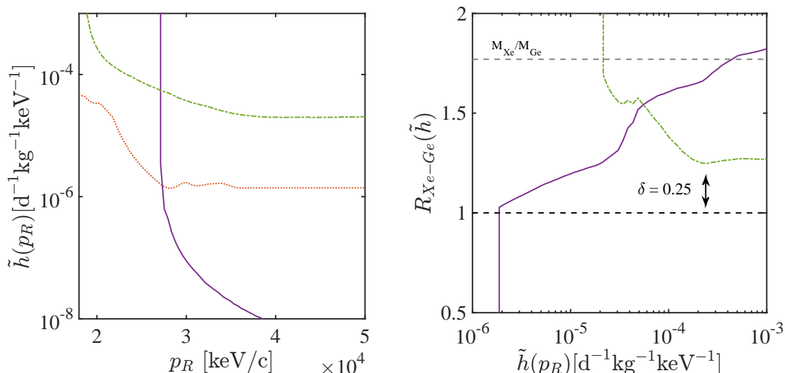
Figure 9. Comparison of exclusion limits without mass assumptions. Left: momentum space exclusion limits from XENON10 (dot-dashed green), LUX (solid purple), and SuperCDMS (dotted orange). Right: ratio of exclusion in p_R -space of LUX to SuperCDMS (solid purple) and XENON10 to SuperCDMS (dot-dashed green). Deviations from monotonicity are smoothed so that the limits \tilde{h}(p_R) can be inverted to form R_{\text{Xe-Ge}}(\tilde{h}) , as in equation (A.1). The minimum value of \delta = 0.25 implies that SuperCDMS is stronger than XENON10 across the full range of v_{\min} only for m_\chi \lesssim 59 GeV. The SuperCDMS and LUX limits, on the other hand, probe complementary ranges of v_{\min} for all DM masses.
