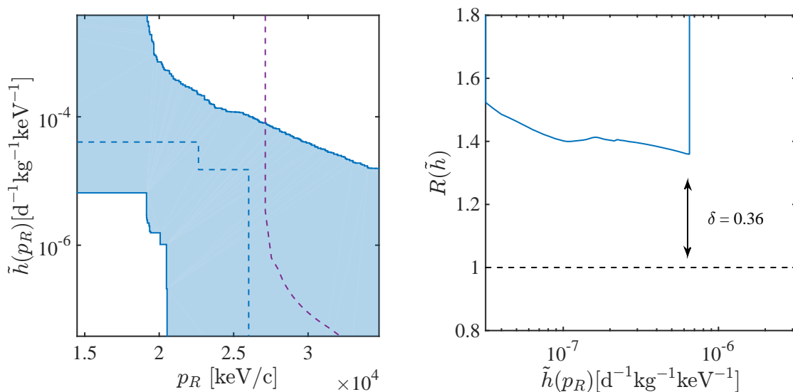
Figure 6. Momentum-space plot comparisons between CDMS II Si and LUX, analogous to figure 5. Left: exclusion limits from LUX (purple) in p_R -space overlaid with preferred region of CDMS II Si (shaded blue) and best fit halo (dashed blue). Right: R -ratio of LUX exclusion with lower boundary of CDMS II Si preferred region. The minimum value of \delta = 0.36 , implies that LUX excludes CDMS II Si across the full range of v_{\min} only for m_\chi \gtrsim 13 GeV.
