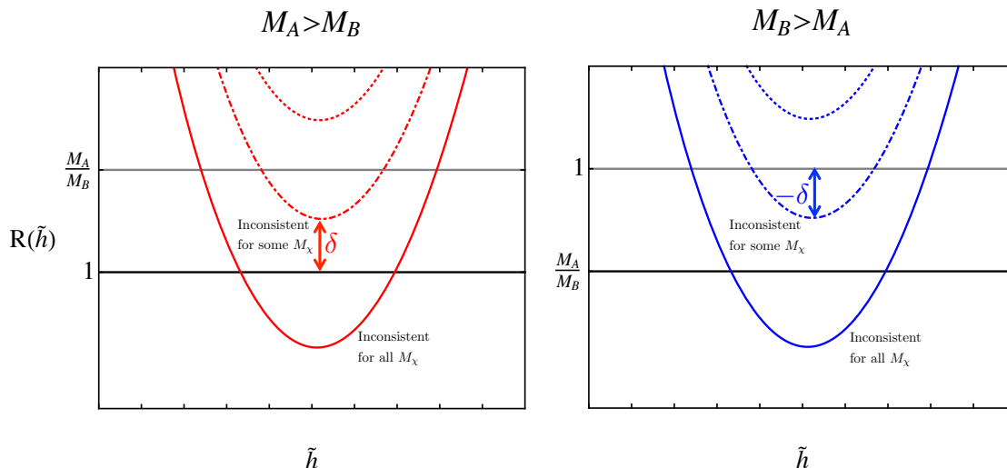
Figure 3. Some possibilities for the variable eq. (3.7), for both possible mass orderings. When moving from p_R -space to v_{\min} -space, the height of any line is rescaled by the DM mass-dependent parameter eq. (3.10) which satisfies the appropriate inequality in eq. (3.11). Case (a) in figure 2 corresponds to the solid red curve, and case (b) corresponds to the dashed or dot-dashed red curves. Cases (c) and (d) cannot be plotted because the lower boundary and the exclusion curve have no overlap in \tilde{h} , and R(\tilde{h}) is undefined.
