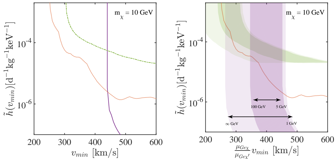
Figure 8. Exclusion limits from XENON10 (dot-dashed green), LUX (solid purple), and SuperCDMS (dotted orange) in v_{\min} -space. Left: v_{\min} -space exclusions for 10 GeV DM. Kinks and slight deviations from monotonicity are present in the SuperCDMS limit, occurring when the “Pmax” method switches the interval used to calculate the exclusion. Similar discrete artifacts are not present in LUX because an observation of zero events is used to calculate the limit, nor in XENON10 because the experiment observed a large number of events. Right: limits with v_{\min} calculated for a range of DM masses and scaled to m_\chi = 10 GeV using the factor appropriate for Ge \mu_{Ge,\chi}/\mu_{Ge,\chi'} , where \mu_{Ge,\chi} is the reduced mass for 10 GeV DM and Ge target. This has the effect of mapping SuperCDMS limits to a single line (dotted orange), independent of mass, while limits from Xe experiments are mapped to different locations depending on the DM mass. Dark bands correspond to the range of limits with masses 5-100 GeV, while the light bands show the range of limits for all possible masses, which facilitates comparison of the relative strengths of the limits for different DM masses.
