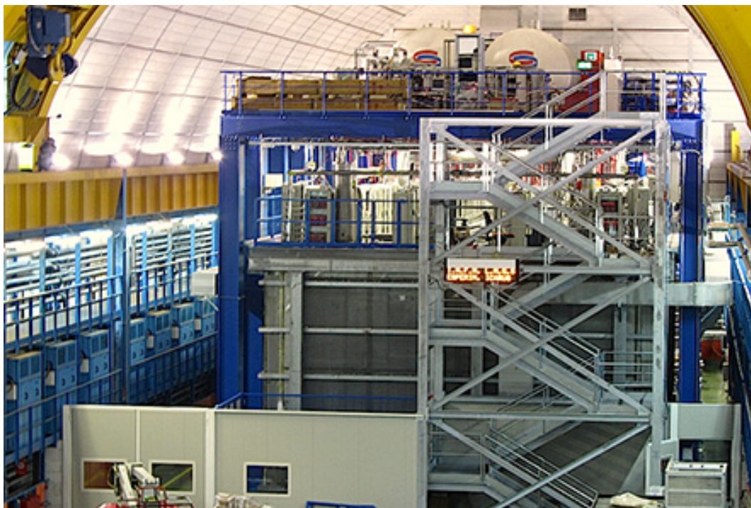
Figure 1. The ICARUS T600 plant in the Northern side of the Hall B at LNGS. Ladders to access the intermediate and the top levels are visible in the front together with the 3 m high wall that separates the T600 area from the rest of Hall B. Cabinets with the readout electronics are installed at the intermediate level. At the top level, the two 30 m 3 cryogenic storage tanks and the additional electronic equipment (HV supply, PMT electronics, trigger system, etc.) are also visible. The cryogenic equipment (nitrogen and argon pumps, cryocoolers, etc.) is located on the rear side of the T600, at the Northern end of the Hall B.
