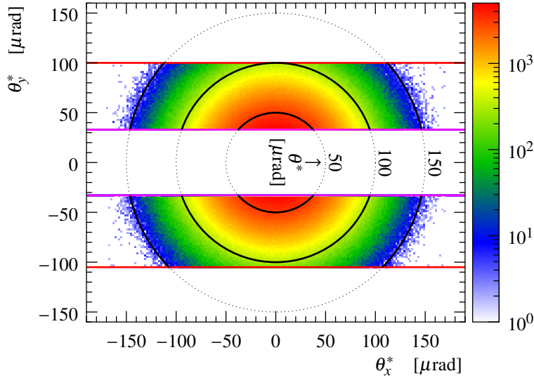
Fig. 5: Distribution of scattering angle projections \theta_y^* vs. \theta_x^* . The upper (lower) part comes from the diagonal 45 bottom – 56 top (45 top – 56 bottom). The colour scale gives number of events (after the \mathcal{A}_{\text{fluct}} correction) per bin. The horizontal lines at \theta_y^* \approx \pm 100 \mu\text{rad} (red) represent cuts due to the LHC apertures, while those at \theta_y^* \approx \pm 30 \mu\text{rad} (magenta) represent cuts due to the sensor edges. The dotted circles show contours of constant scattering angle \theta^* as indicated in the middle of the plot. The parts of the contours within acceptance are emphasised in thick black. (For interpretation of the references to colour in this figure legend, the reader is referred to the web version of this article.)
