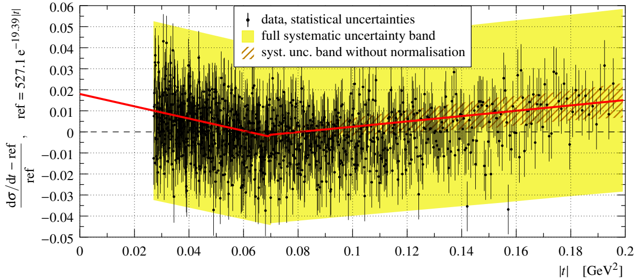
Fig. 12: Differential cross-section using the “per-mille” binning and plotted as relative difference from the reference exponential (see vertical axis). The black dots represent data points with statistical uncertainty bars. The red line (with two straight segments) shows pure exponential fits in regions below and above |t| = 0.07 \text{ GeV}^2 , see Eq. (19). The widest error band (yellow) corresponds to the full systematic uncertainty, the hatched one (brown) includes all systematic contributions except the normalisation. Both bands are centred around the fit curve. (For interpretation of the references to colour in this figure legend, the reader is referred to the web version of this article.)
