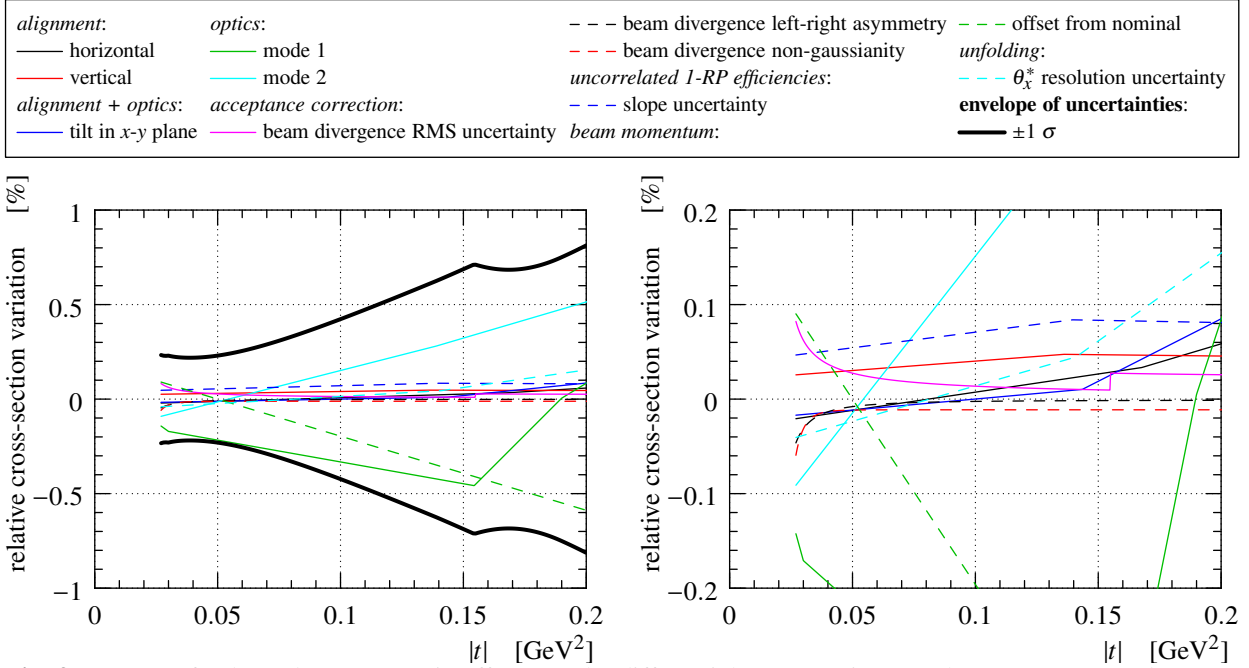
Fig. 9: Impact of t -dependent systematic effects on the differential cross-section. Each curve corresponds to a systematic error at 1 \sigma , cf. Eq. (13). The two contributions due to optics correspond to the two vectors in Eq. (8). The envelope is determined by summing all shown contributions in quadrature for each |t| value. The right plot provides a vertical zoom; note that the envelope is out of scale.
