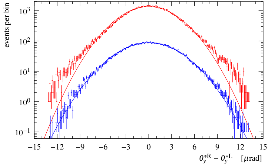
Fig. 1: Difference between vertical scattering angles reconstructed in the right and left arm, for the diagonal 45 bottom - 56 top. Upper graph (red): data from run start (0.5 to 1.5h from the beginning of the run). Lower graph (blue): data from run end (10.5 to 11.5h), scaled by 0.1. The solid lines represent Gaussian fits.
