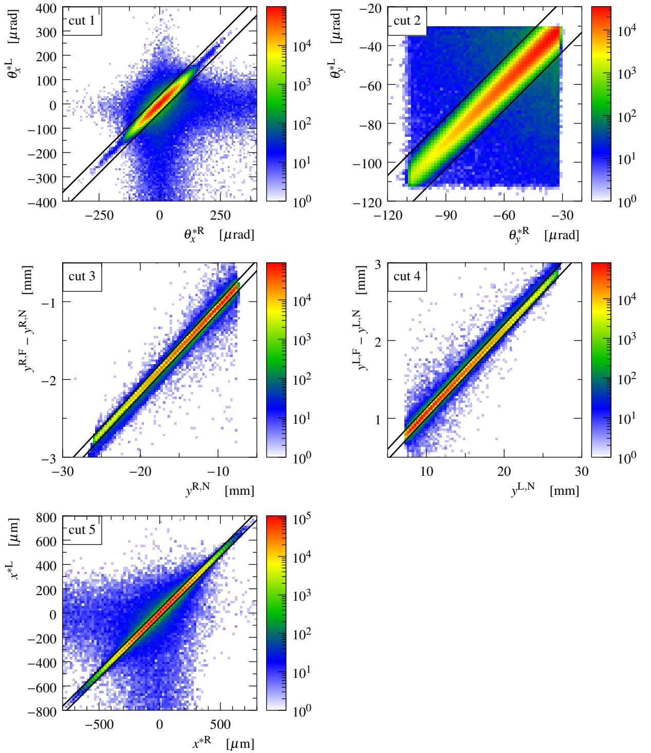
Fig. 3: Correlation plots for the event selection cuts summarised in Table 2, using all events with diagonal topology 45 top – 56 bottom. The black solid lines delimit the signal ( \pm 4\sigma ) region.
