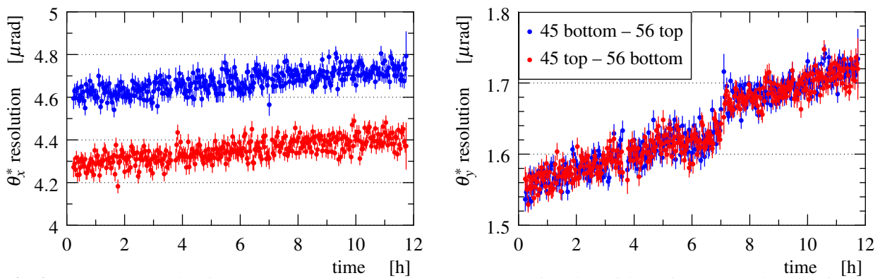
Fig. 2: Angular resolution for the two-arm reconstruction, Eq. (4), as a function of time (from the beginning of the run). The step in \theta_y^* resolution around 7h is due to inclusion of another colliding bunch-pair with a larger vertical emittance.
