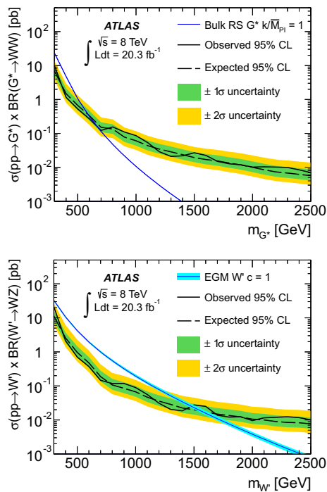
Fig. 2 Observed and expected 95 % CL upper limits on the cross section times branching fraction as a function of the resonance pole mass for the G^* (top) and EGM W' (bottom). The LO (NNLO) theoretical cross section for the G^* ( EGM W' ) production is also shown. The inner and outer bands around the expected limits represent \pm 1\sigma and \pm 2\sigma variations respectively. The band around the W' cross section corresponds to the NNLO theory uncertainty
