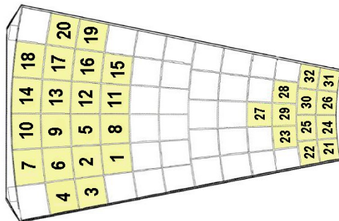
Figure 4. Schematic drawings of a GaAs sensor. Each of the 32 connected pads is identified by a number.
