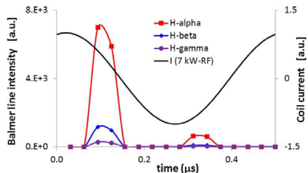
Figure 2: Simulated plasma light emission at plasma ignition, the phase of the RF-current passing through a 6 turns solenoid is indicated.
