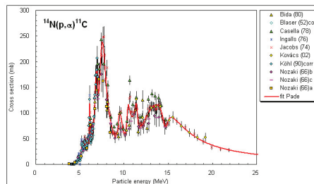
Figure 1: Cross section for 11 C production, from [3]
