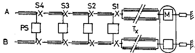
Fig. 7. Schematic of eight pulse burst generator.
