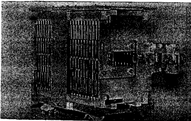
Fig. 10. 24 cell PS injection kicker magnet module.
