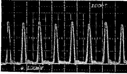
Fig. 8. Eight pulse burst current after magnet traversal.
