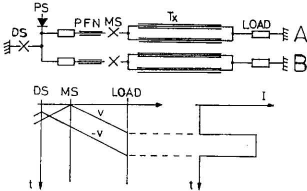
Fig. 3. EPA injection generator schematic with pulse derivation.
