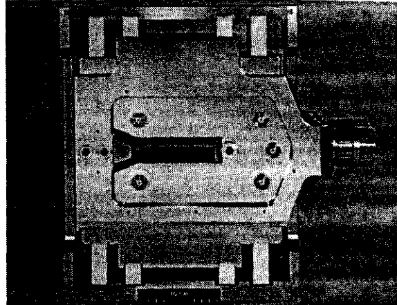
Fig. 2. 7 cell EPA injection kicker magnet module.
