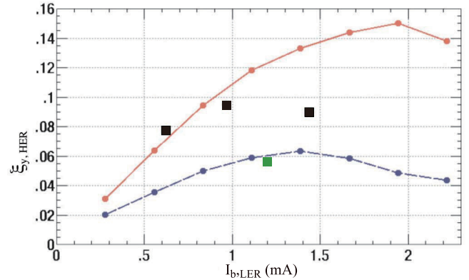
Figure 2: Predicted beam–beam parameters obtained from strong–strong beam–beam simulations with crossing angle 22 mrad (purple) and for head-on or crab crossing (red). Some experimental data are also shown (squares), with black and green squares representing data with and without the crab cavities, respectively.
