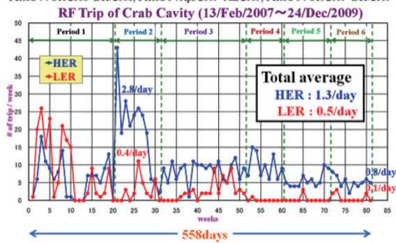
Figure 7: Trip rate of crab cavity system.
