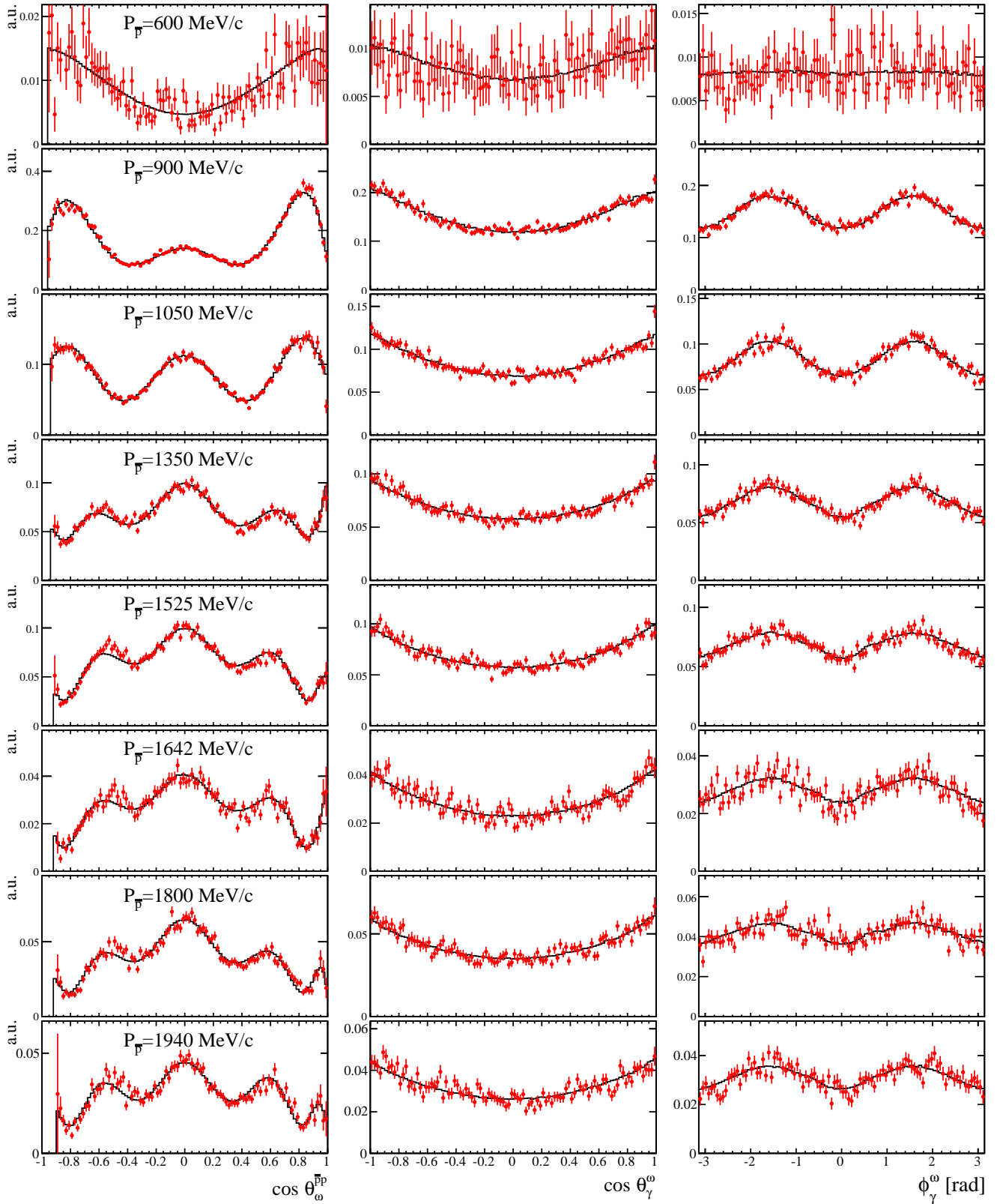
Fig. 5 Acceptance corrected angular distributions for the channel \bar{p}p \rightarrow \omega\pi^0 \rightarrow (\pi^0\gamma)\pi^0 as a function of the production angle (first column) and of the decay angle in \cos(\theta_{\gamma}^{\omega}) (second column) and \phi_{\gamma}^{\omega} (third column). The production angle is defined in the \bar{p}p rest frame by the direction of the \omega related to the beam axis. The decay angles are specified by the helicity system of the \omega meson. The production angle distribution is given integrated over all \omega -decay angles, the decay angle distributions are given integrated over all production angles. While the data are marked with red error bars, the fit results (Sec. 4) are plotted with black lines. Each row represents one specific beam momentum.
