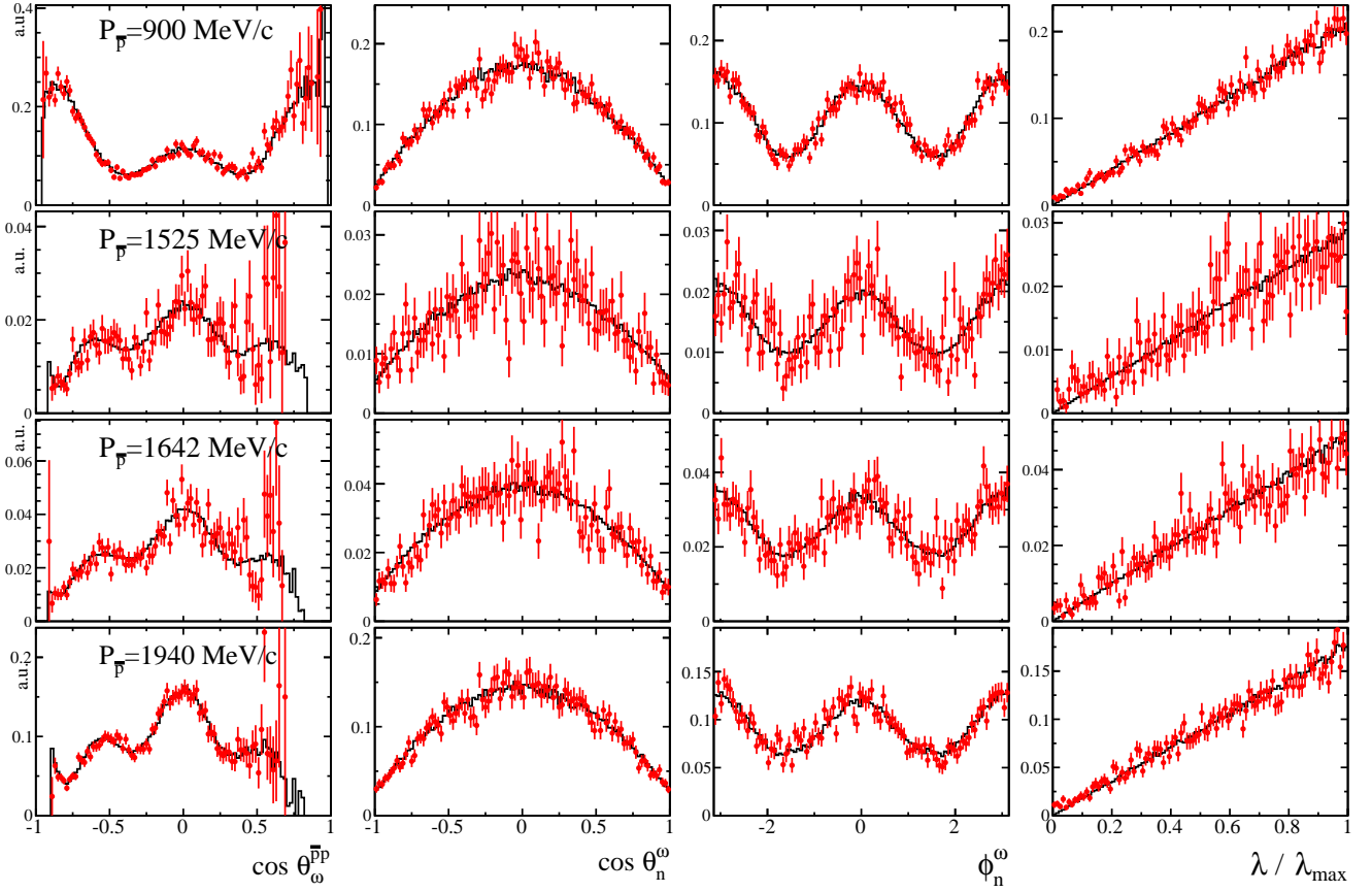
Fig. 6 Acceptance corrected angular distributions for the channel \bar{p}p \rightarrow \omega\pi^0 \rightarrow (\pi^+\pi^-\pi^0)\pi^0 as a function of the production angle \cos(\theta_{\bar{p}}^{\omega}) (first column) and of the decay angle in \cos(\theta_n^{\omega}) (second column) and \phi_n^{\omega} (third column). The production angle is defined in the \bar{p}p rest frame by the direction of the \omega related to the beam axis. The decay angles \theta_n^{\omega} and \phi_n^{\omega} are specified by the normal of the decay plane of the \omega meson in its helicity system. The production angular distribution is integrated over all \omega -decay angles, the decay angular distributions are integrated over all production angles. The fourth column represents the normalized transition rate \lambda of the \omega decay. A detailed description of this property can be found in sec. 3.1. While the data are marked with red error bars, the fit results (Sec. 4) are plotted with black lines. Each row represents one specific beam momentum.
