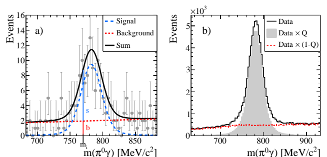
Fig. 3 a) Invariant \pi^0\gamma mass from a data subset of the 200 nearest neighbors associated to a certain \pi^0\pi^0\gamma event at the beam momentum of 900 MeV/c. The black shape represents the complete fit result for the determination of the event weight. The dashed blue line shows the obtained content of the \omega signal and the red dotted line the fraction of the background contribution. b) Invariant \pi^0\gamma mass of all selected \pi^0\pi^0\gamma events at 900 MeV/c. The shaded area represents the signal fraction where each event is weighted by its Q -value. The background content with the individual event weight of (1-Q) is marked with the dotted red line.
