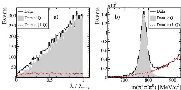
Fig. 4 Histogram (a) shows the normalized transition rate \lambda/\lambda_{max} of the \omega decay. Histogram (b) represents the invariant \pi^+\pi^-\pi^0 mass of all selected \pi^+\pi^-\pi^0 events at the beam momentum of 900 MeV/c. The excellent background separation power can be seen by the shaded areas representing the fraction of the signal events and the dotted red lines illustrating the background content.
