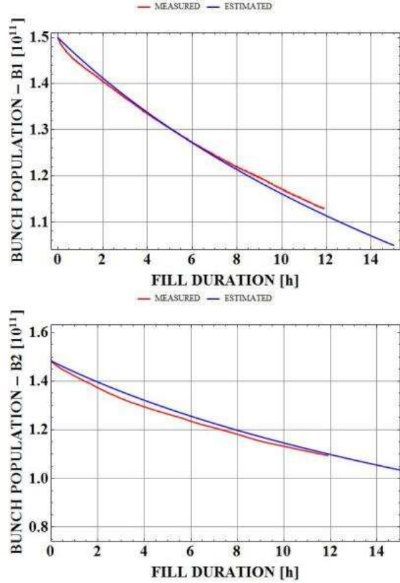
Figure 4. Average bunch population evolution measured (red) during fill 2728 for beam 1 (top) and beam 2 (bottom) compared with the evolution estimated with the model above described (blue).
