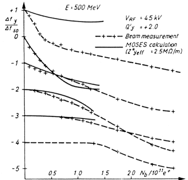
Fig. 4: Shift with the intensity of the Theoretical Modes of a Positron Single Bunch Beam
