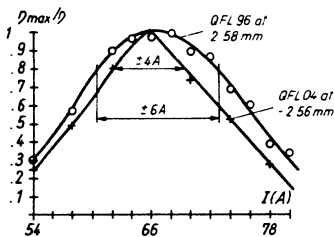
Fig. 5 MARGINS at injection for two different closed orbit corrections
