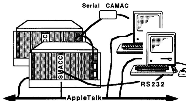
Fig 4 - MacinSMACC
