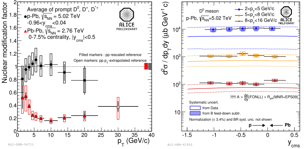
Fig. 1. Left panel: comparison of average D^0 , D^{*+} and D^+ nuclear modification factors measured in p–Pb collisions and in the 0–7.5% most central Pb–Pb collisions. Right panel: p_T , y -differential cross-section for D^0 production in p–Pb collisions as a function of the rapidity in the centre of mass system for three different p_T ranges. The continuous and dashed lines represent expectations based on pQCD calculations including EPS09 parametrization of nuclear PDF [15, 24,22] (see text for more details).
