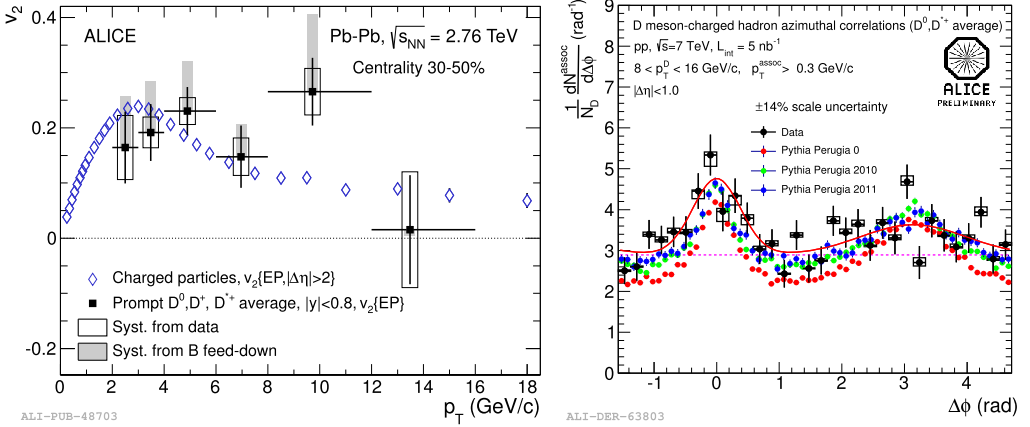
Fig. 3. Left panel (from [28]): comparison between D^0, D^{*+} and D^+ average v_2 and charged hadron v_2 measured in 30–50% central Pb–Pb collisions. Right panel: azimuthal correlations between D mesons (average of D^0 and D^{*+} results) and charged hadrons in pp collisions at \sqrt{s} = 7 TeV, compared to expectations from simulations with the PYTHIA event generator [32,33]. The boxes represent the systematic uncertainty not correlated in \Delta\phi .
