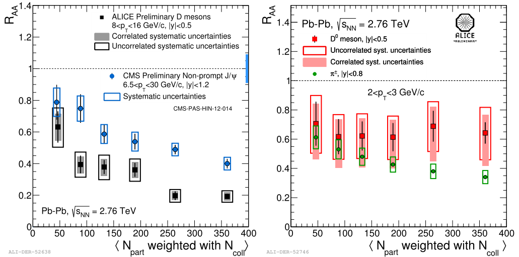
Fig. 2. Comparison of the centrality dependence of the nuclear modification factors of non-strange D mesons in 8 < p_T < 16 \text{ GeV/c} and J/\psi from B-meson decays measured with CMS [26] in 6 < p_T < 30 \text{ GeV/c} (left panel) and of non-strange D mesons and charged pions in 2 < p_T < 3 \text{ GeV/c} (right panel). The filled boxes represent the D-meson systematic uncertainties that are correlated in the different centrality intervals.
